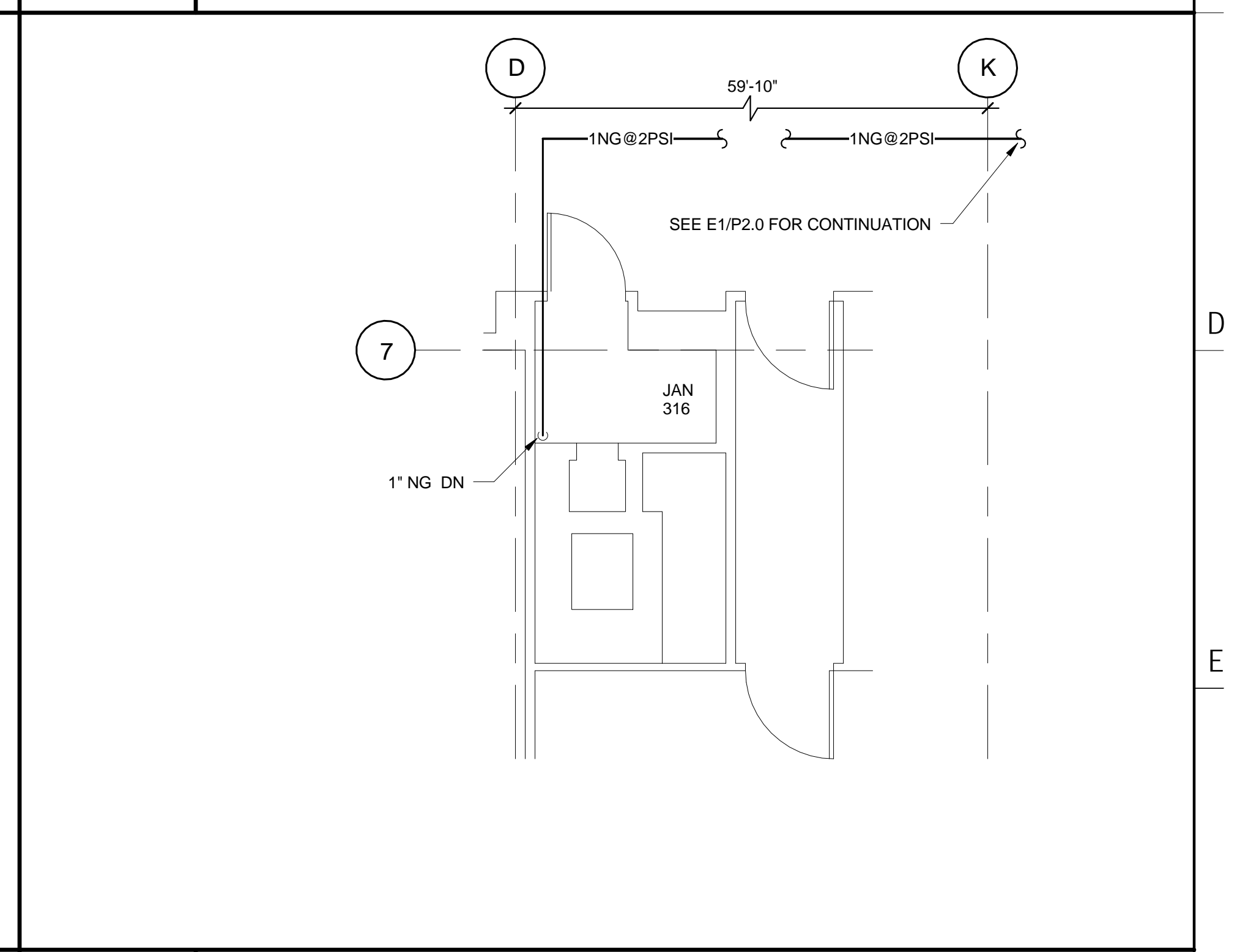
F11 THIRD FLOOR PART PLAN - SUPPLY 1/4" = 1'-0"
