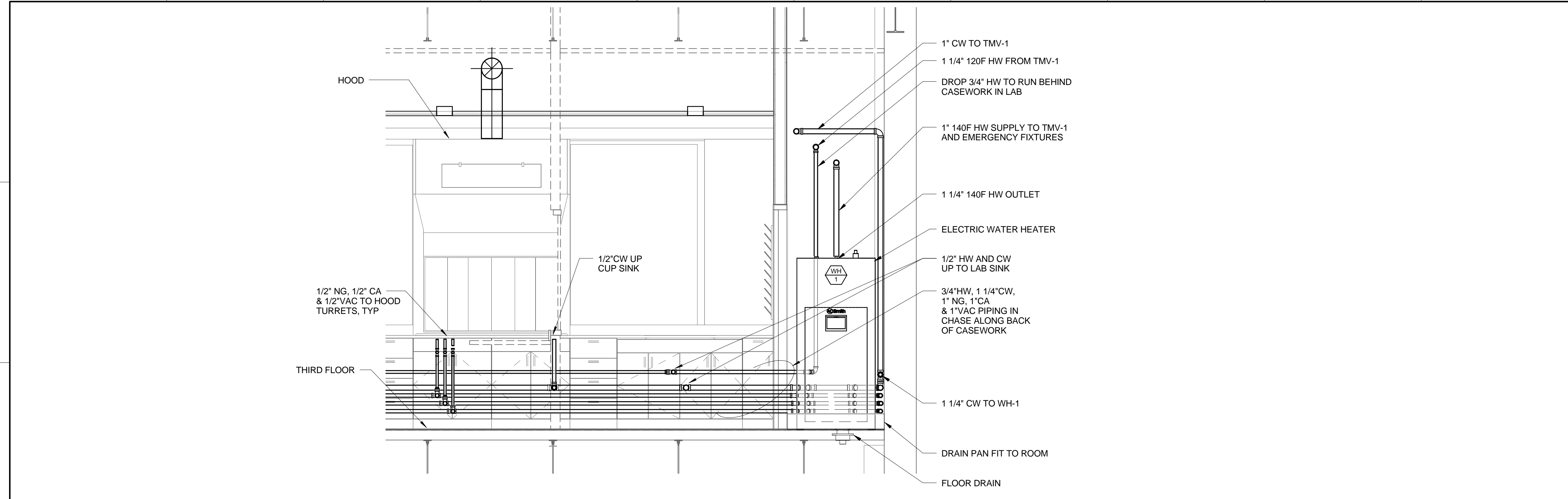
C1 SUPPLY PIPING IN CHASE BEHIND LAB CASEWORK 1/2" = 1'-0"
