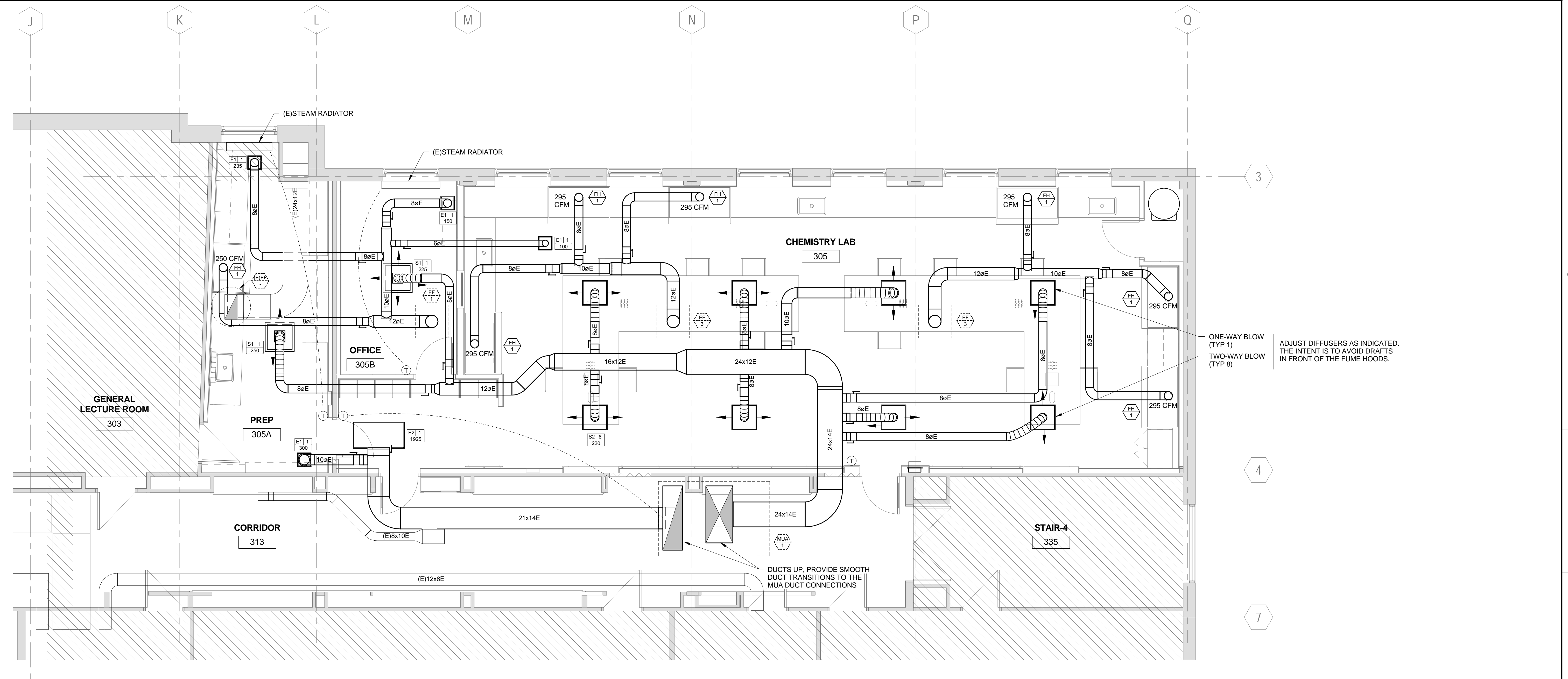
J1 THIRD FLOOR PLAN - HVAC1 1/4" = 1'-0"
