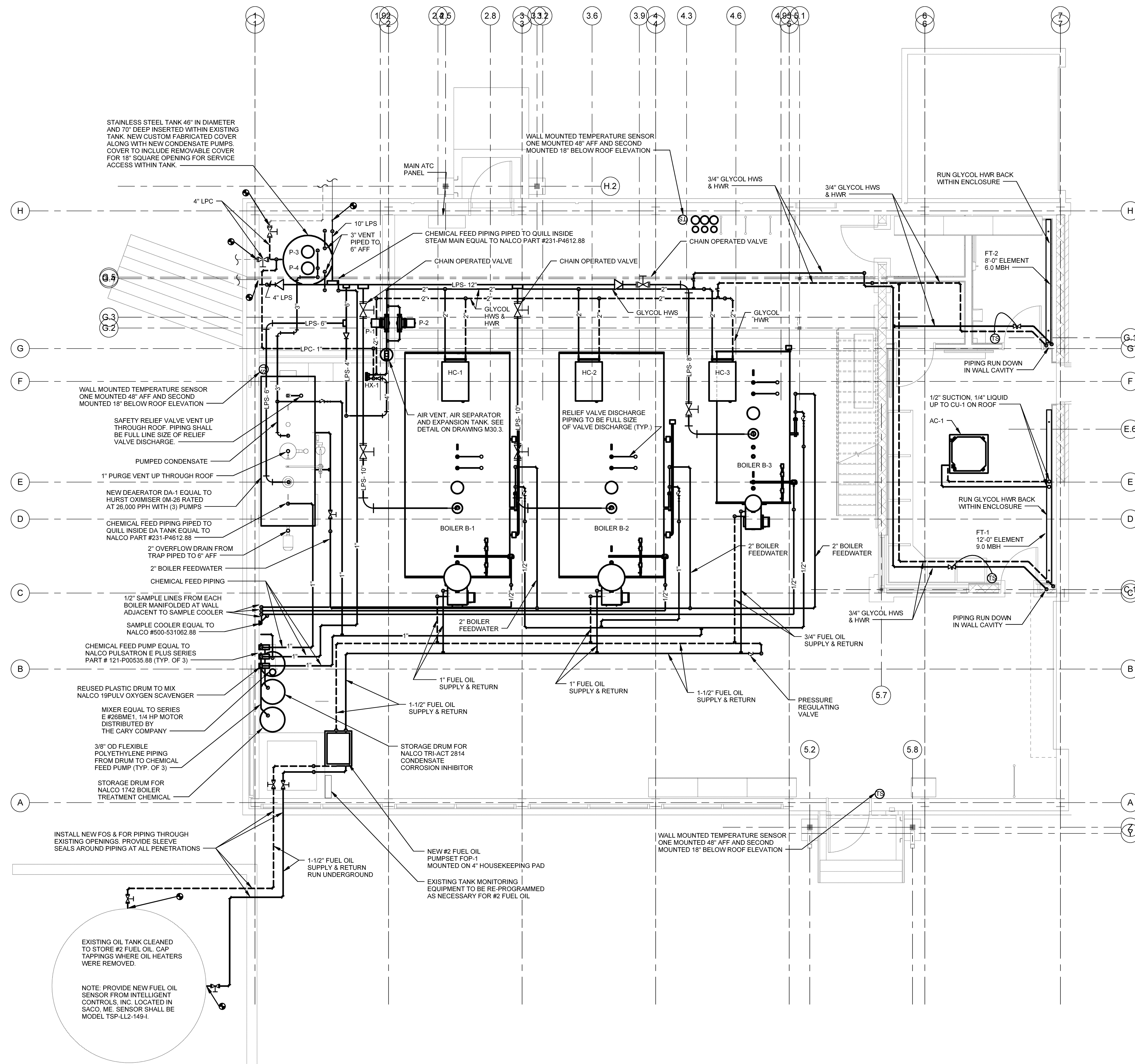
1 FIRST FLOOR PIPING SCALE: 1/4" = 1'-0"
