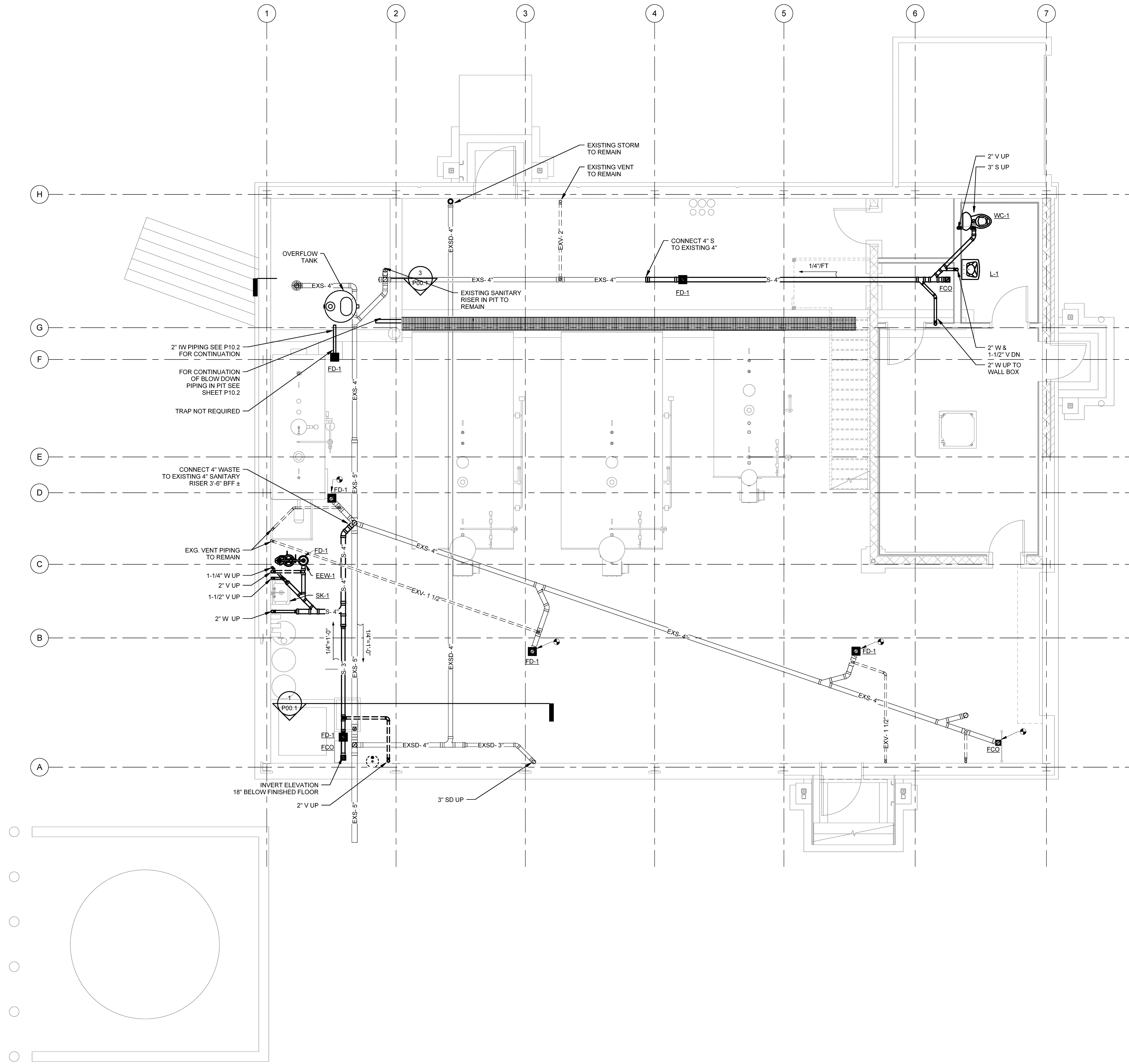
1 FIRST FLOOR UNDERSLAB DRAINAGE SCALE: 1/4" = 1'-0"
