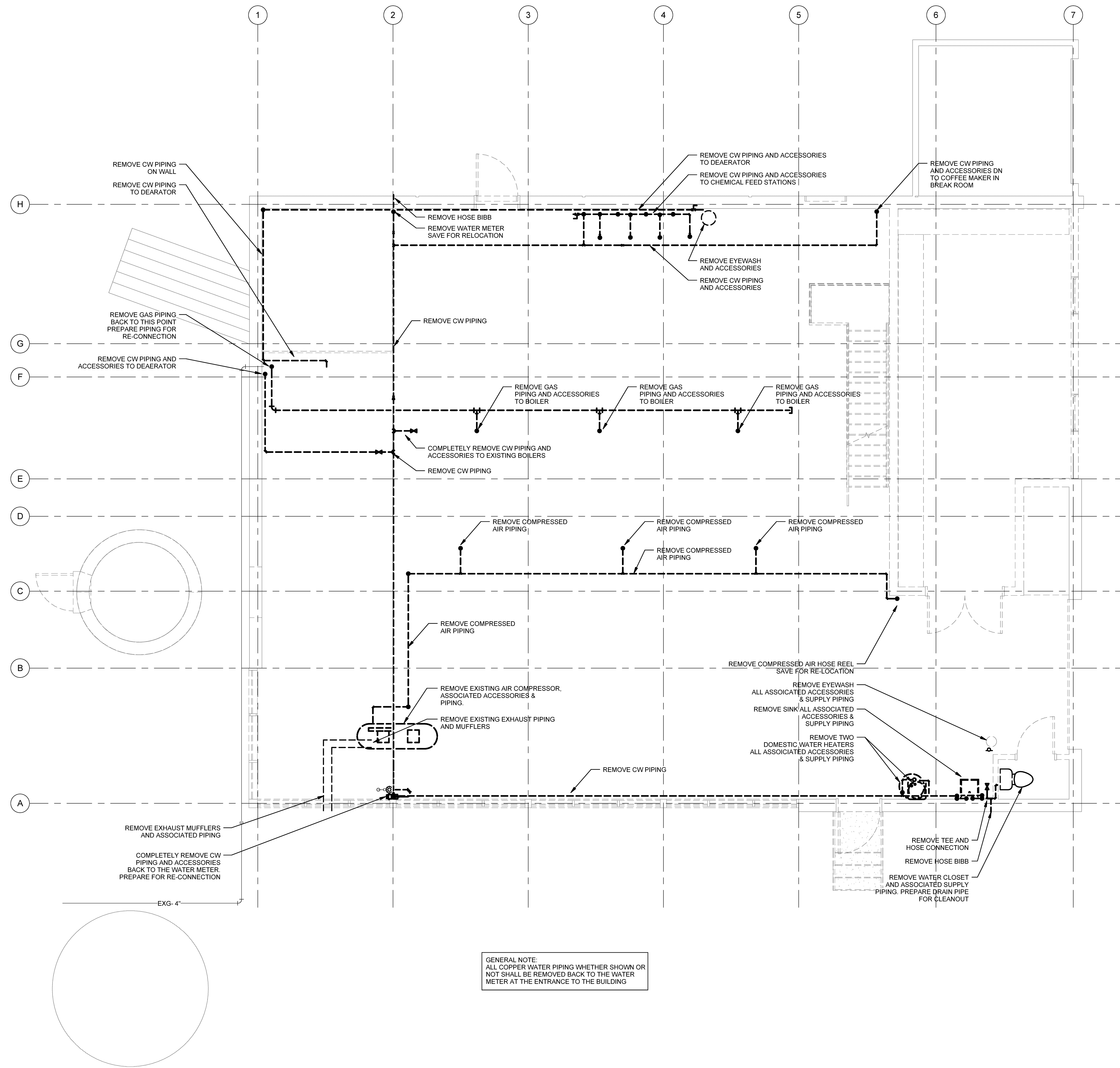
1 FIRST FLOOR DEMOLITION SUPPLY SCALE: 1/4" = 1'-0"
