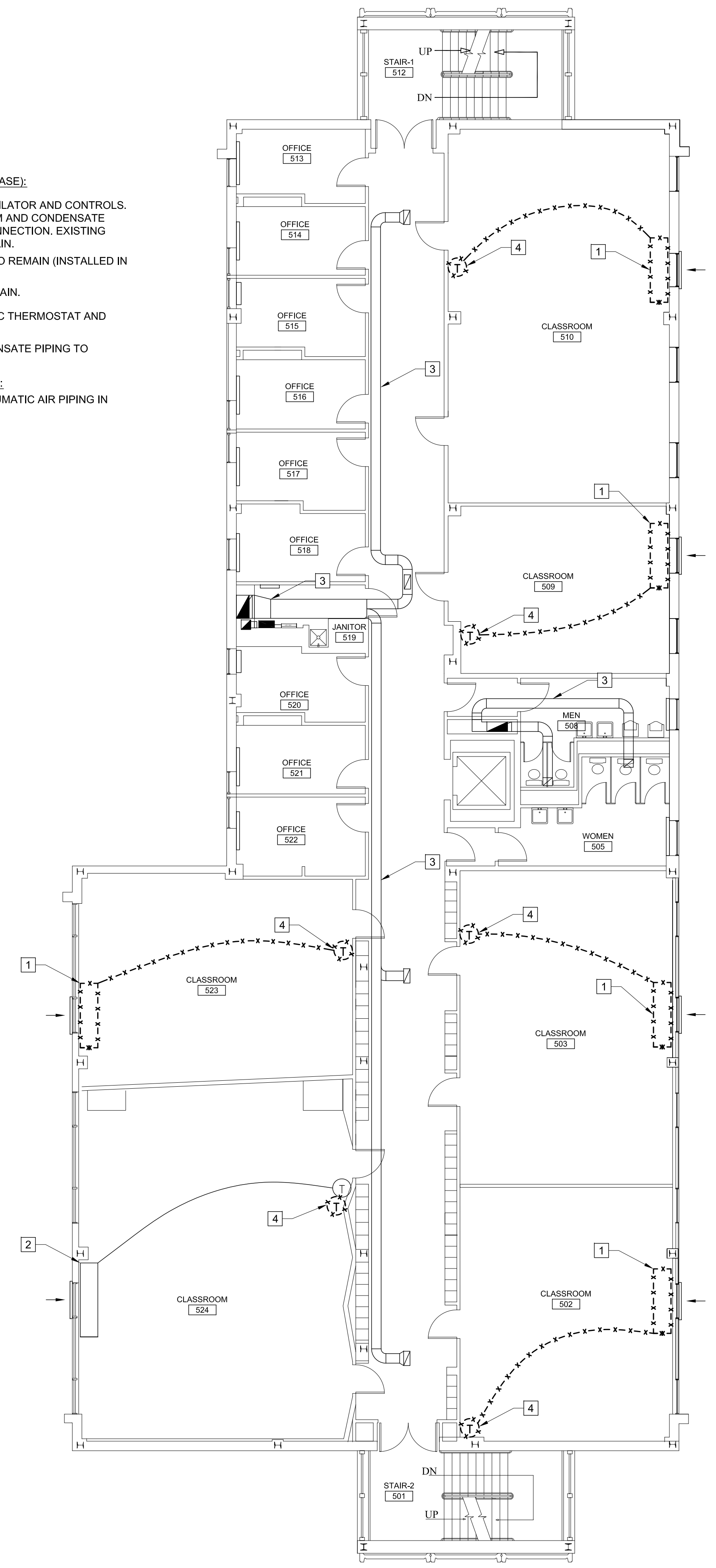
A3 MECHANICAL DEMOLITION FIFTH FLOOR PLAN 1/8"=1'-0"
