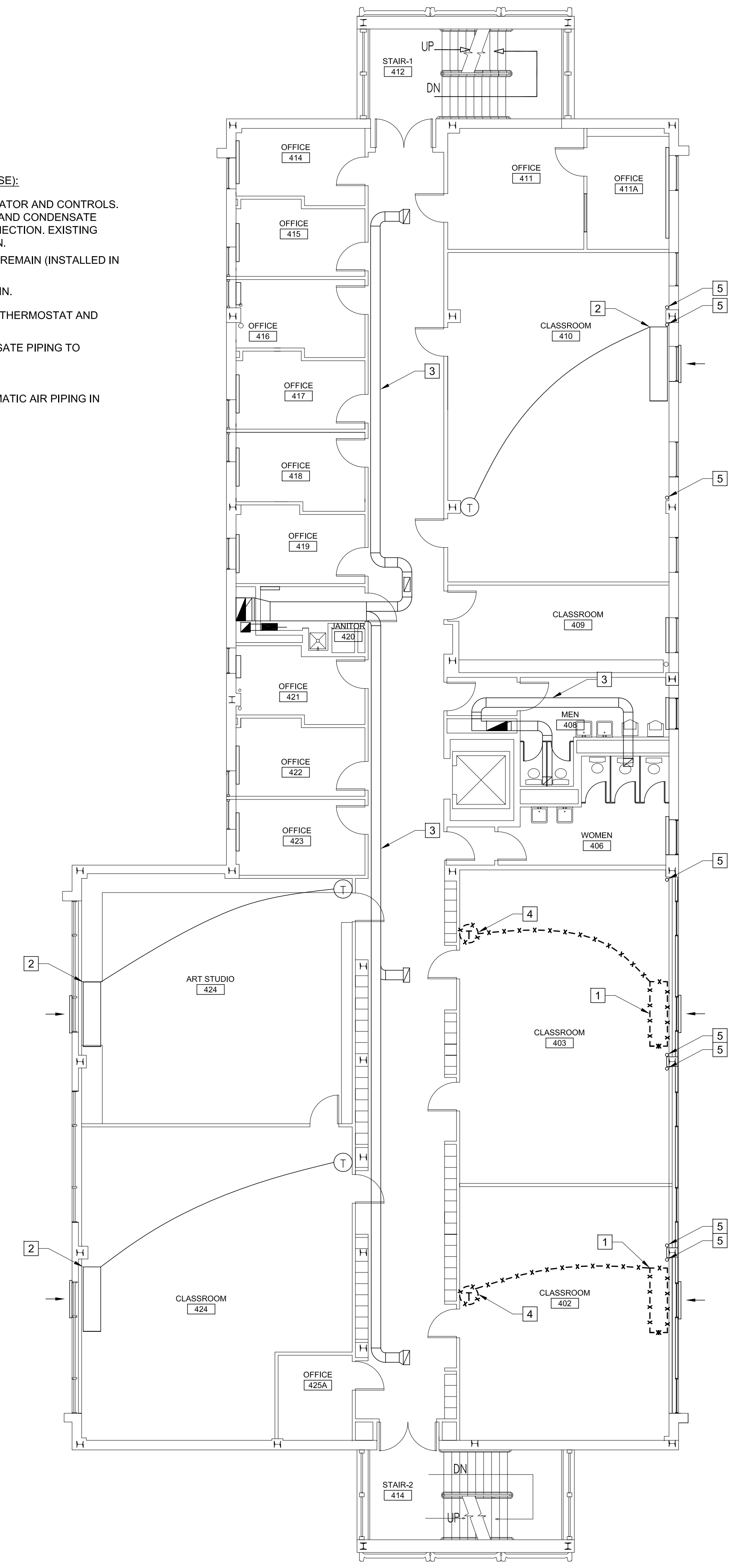
A1 MECHANICAL DEMOLITION FOURTH FLOOR PLAN 1/8"=1'-0"
