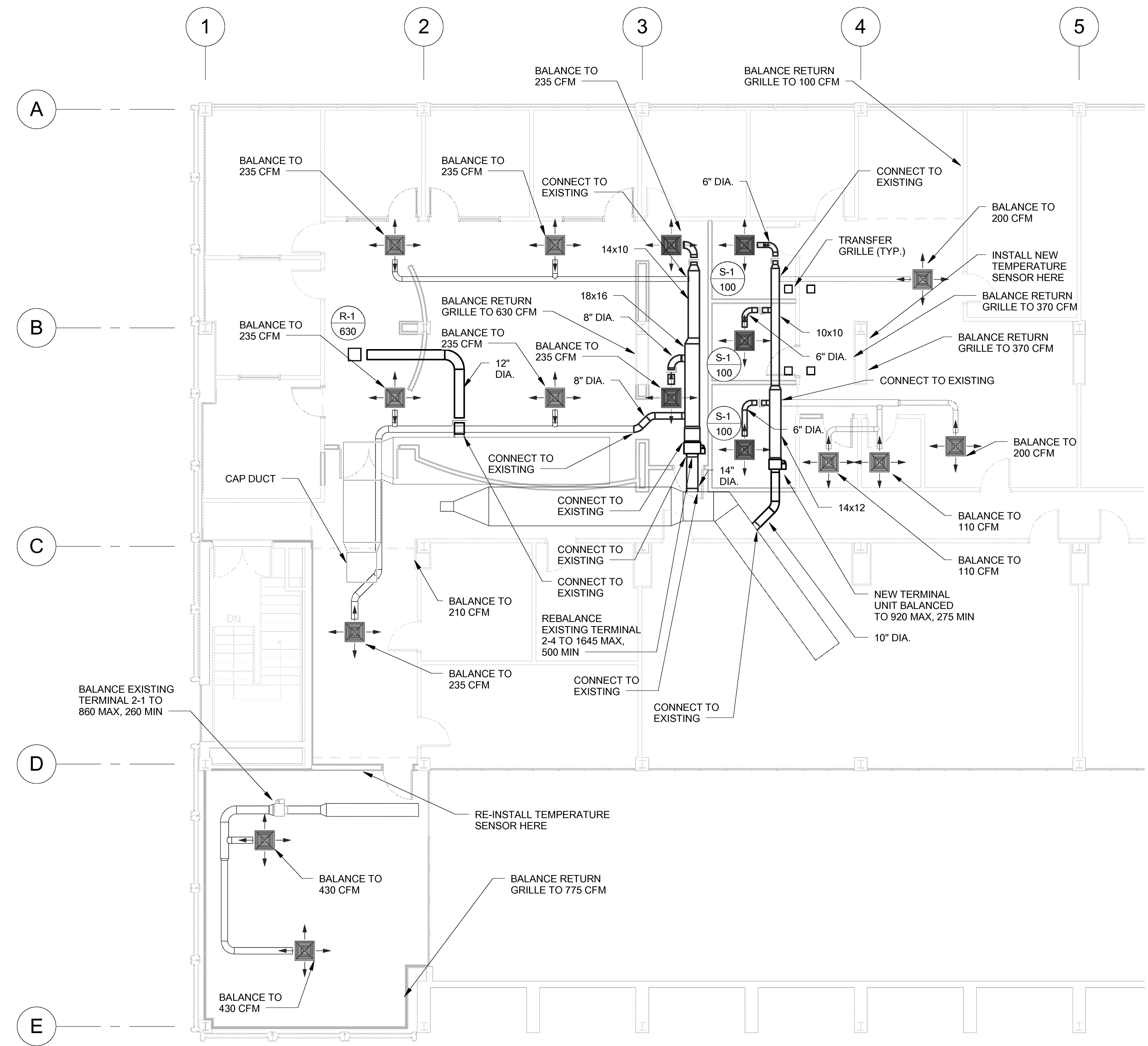
1 M10-2 Ductwork Level 2 SCALE: 1/8" = 1'-0"
