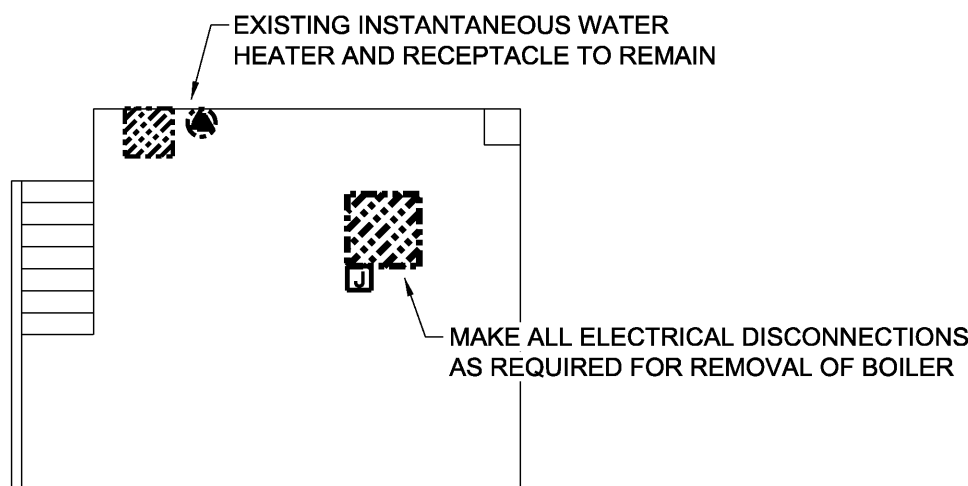
BASEMENT PLAN
