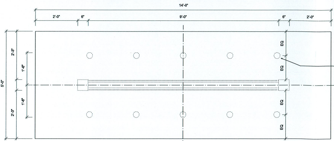
PLAN - Top View SCALE: 3/8"=1'-0"
