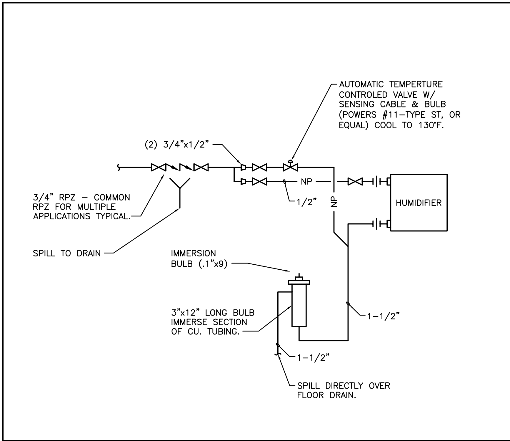
A8 HUMIDIFIER CONNECTION DETAIL NOT TO SCALE
