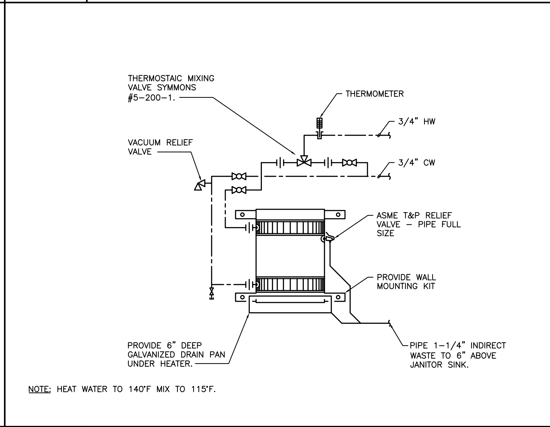
A13 ELECTRIC WATER HEATER DETAIL NOT TO SCALE
