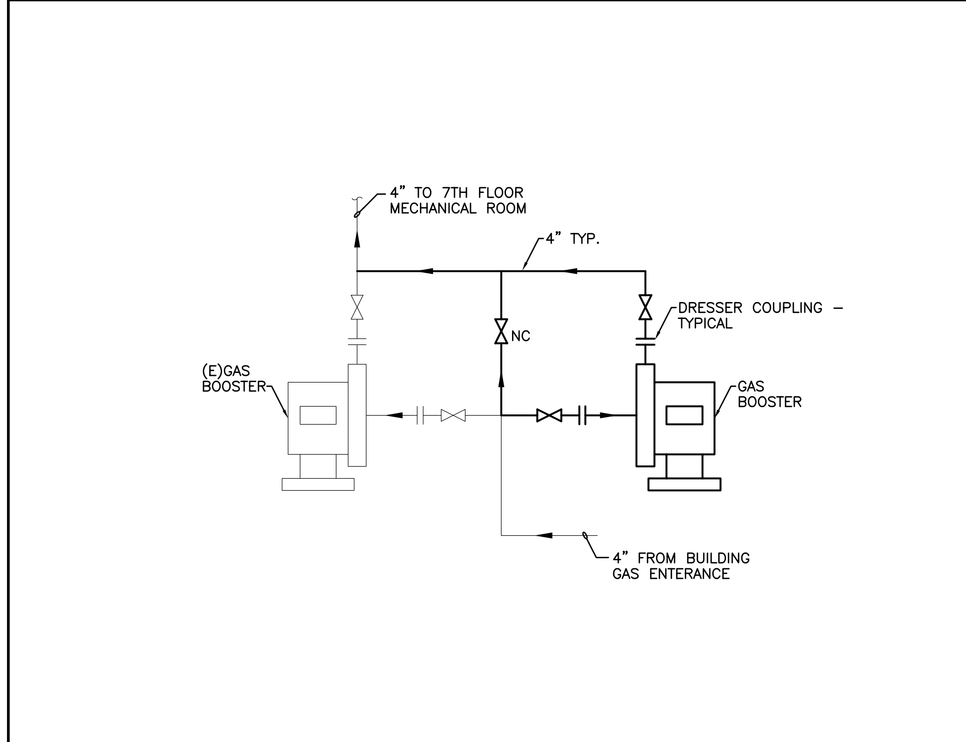
F13 GAS BOOSTER (ADD ALTERNATE #8) NOT TO SCALE
