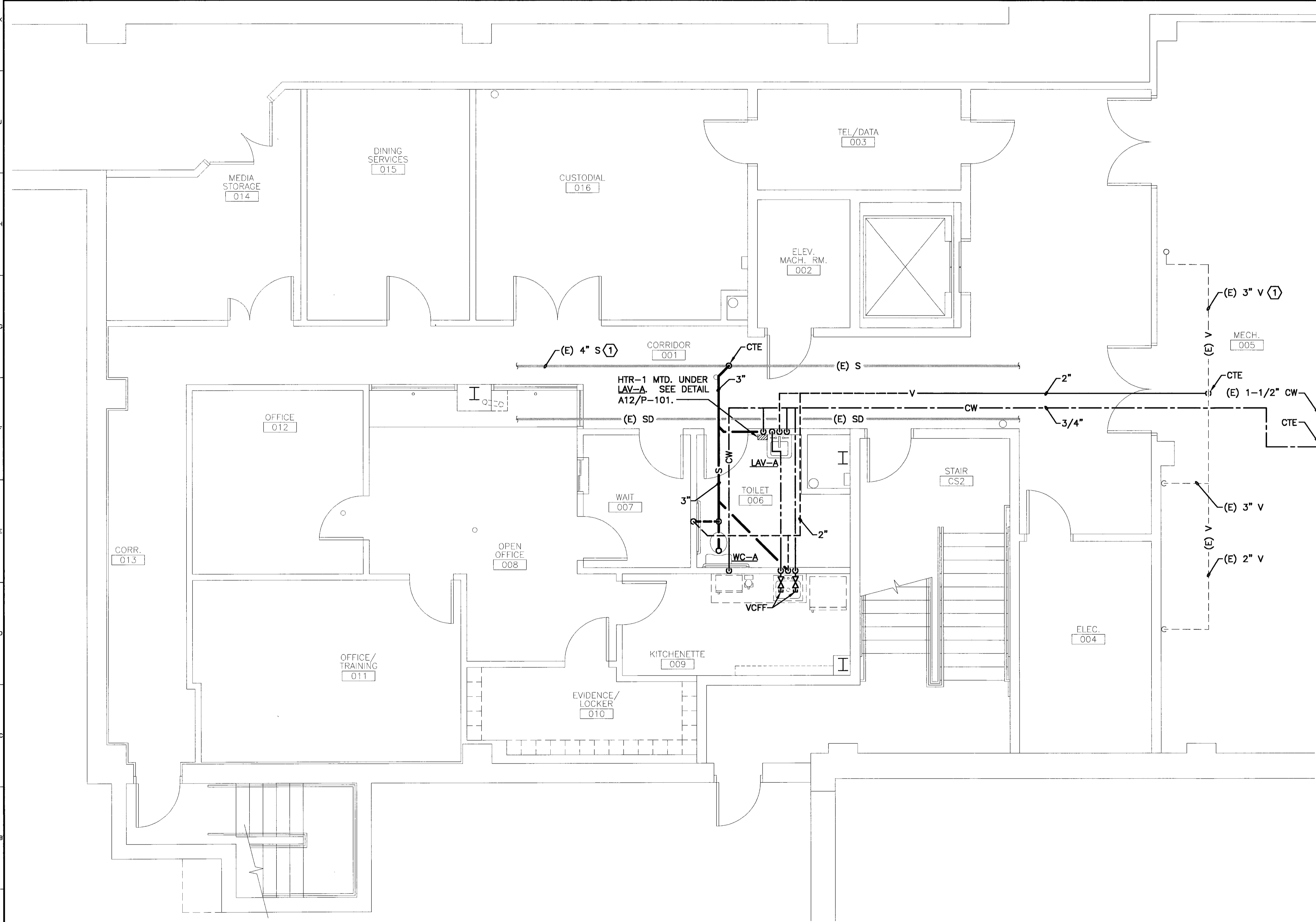
A1 BASEMENT PLAN 1/4" = 1'-0"
