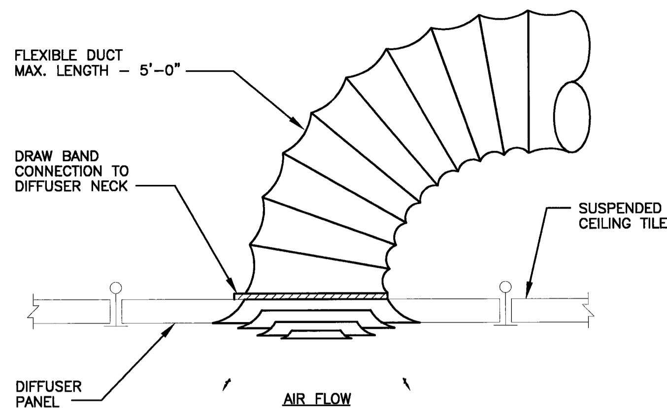
K10 FLEXIBLE DUCT
