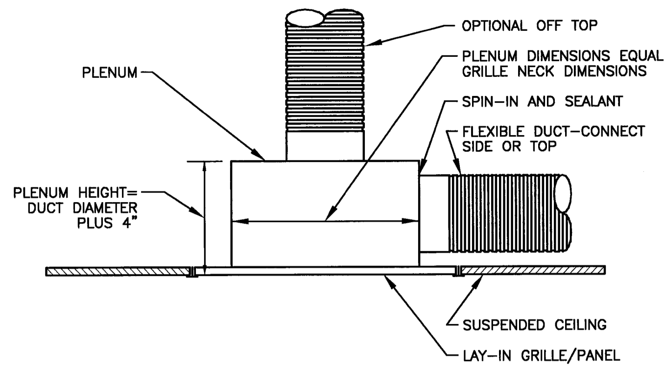
K5 TYP. RETURN & TRANSFER GRILLE PLENUM
