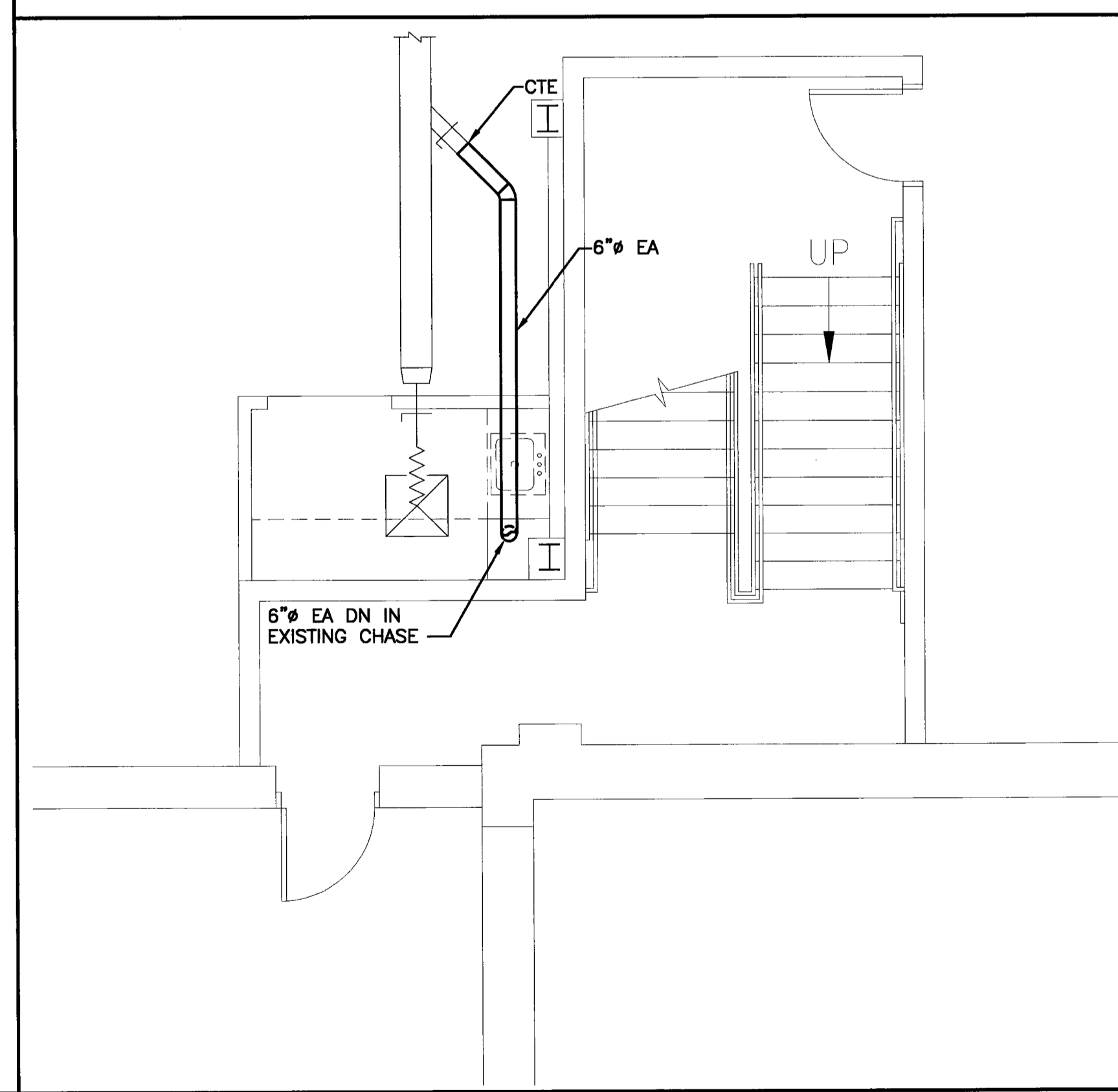
A12 FIRST FLOOR PLAN
