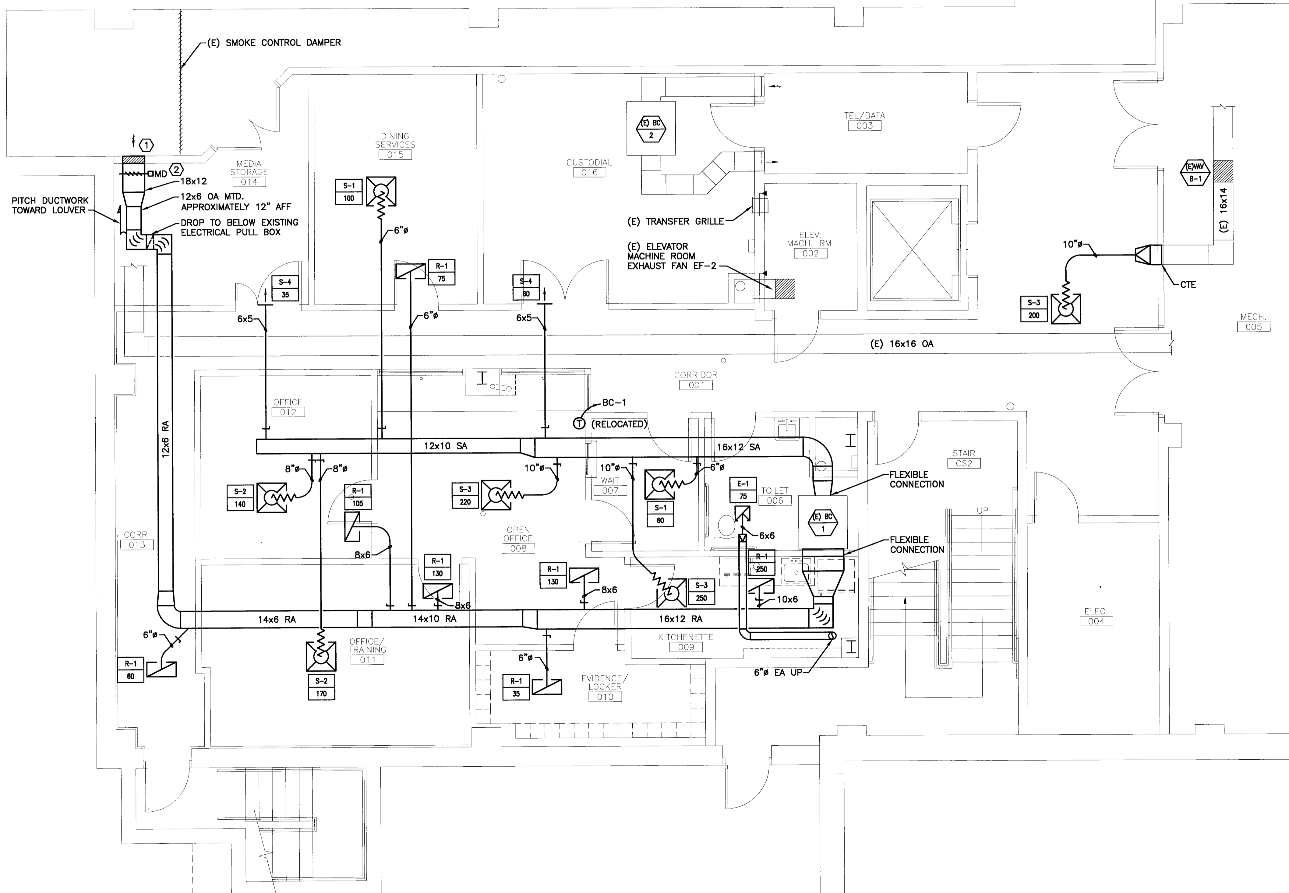
A1 BASEMENT PLAN
