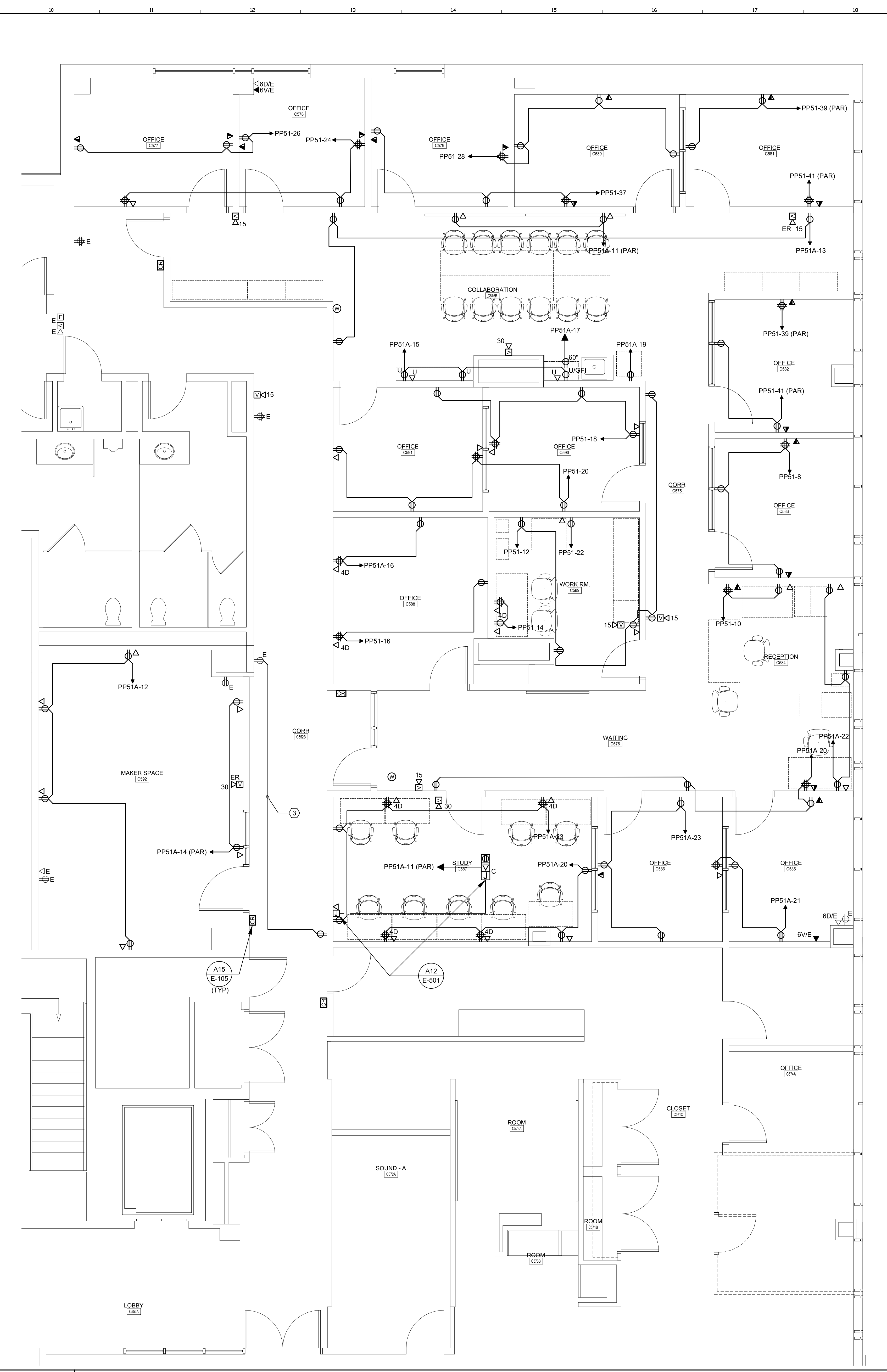
A10 FIFTH FLOOR ENLARGED POWER PLAN 1/4" = 1'-0"
