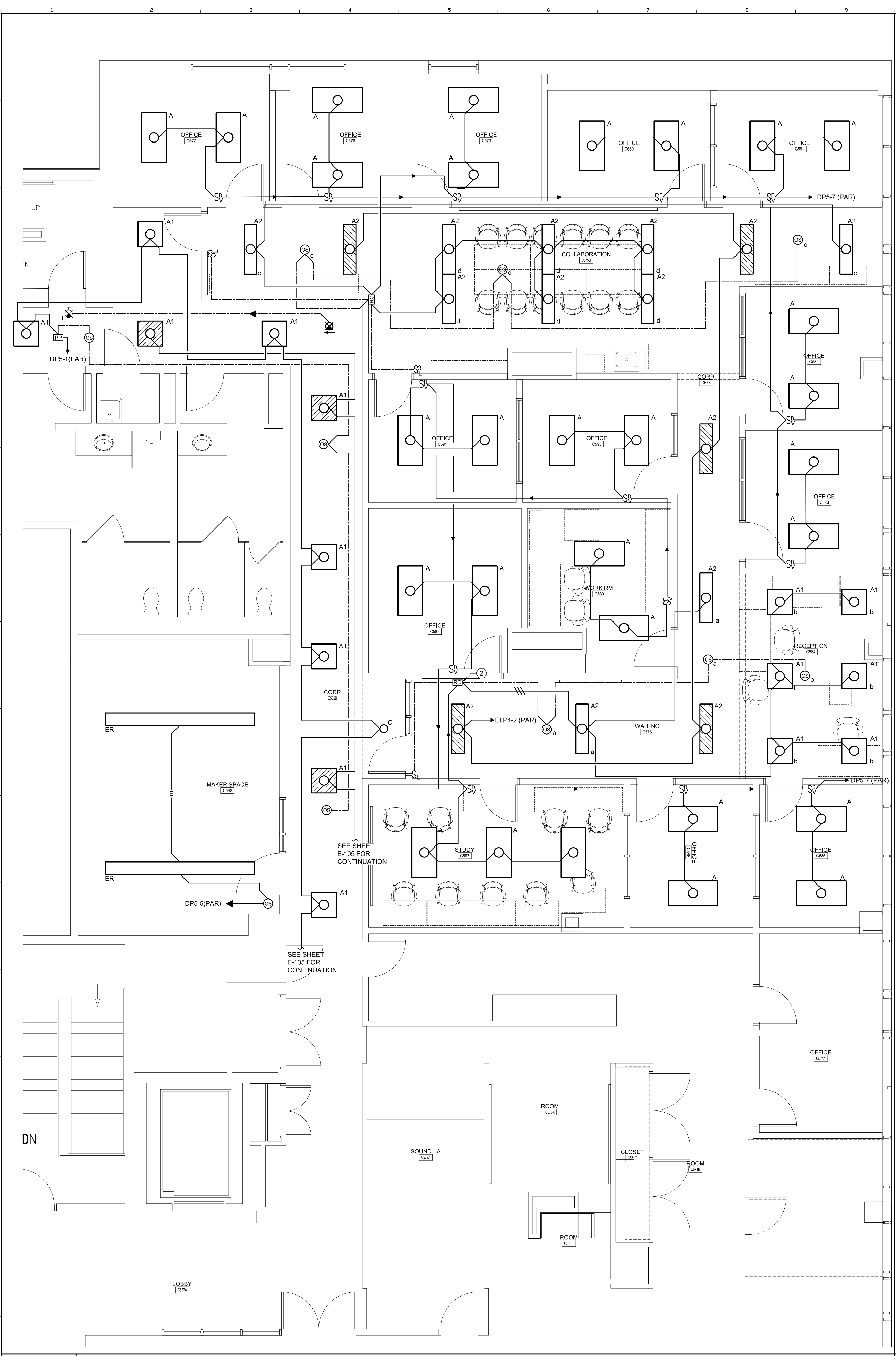
A1 FIFTH FLOOR ENLARGED LIGHTING PLAN 1/4" = 1'-0"
