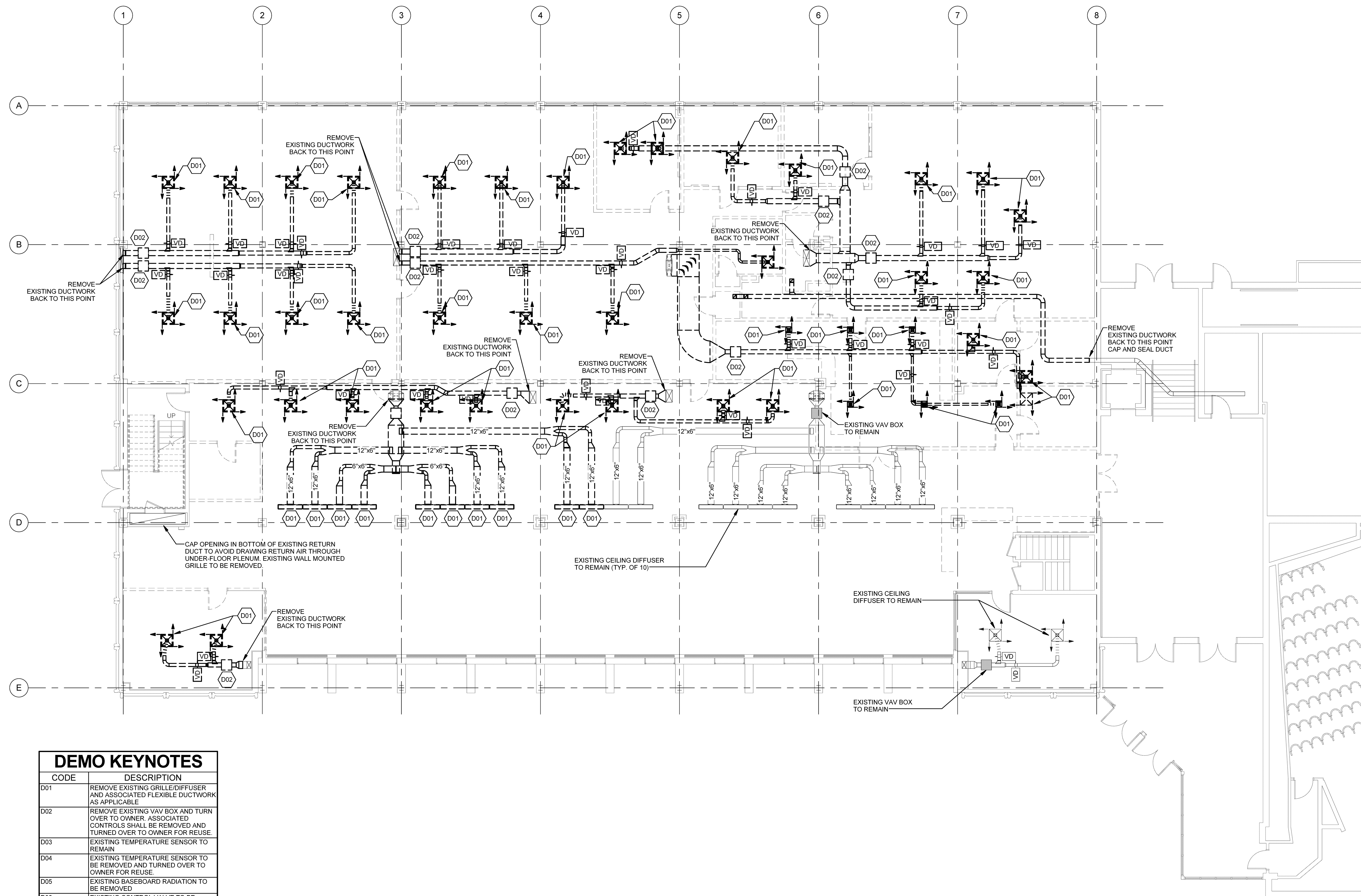
1 DEMOLITION DUCTWORK FIRST FLOOR SCALE: 1/8" = 1'-0"
