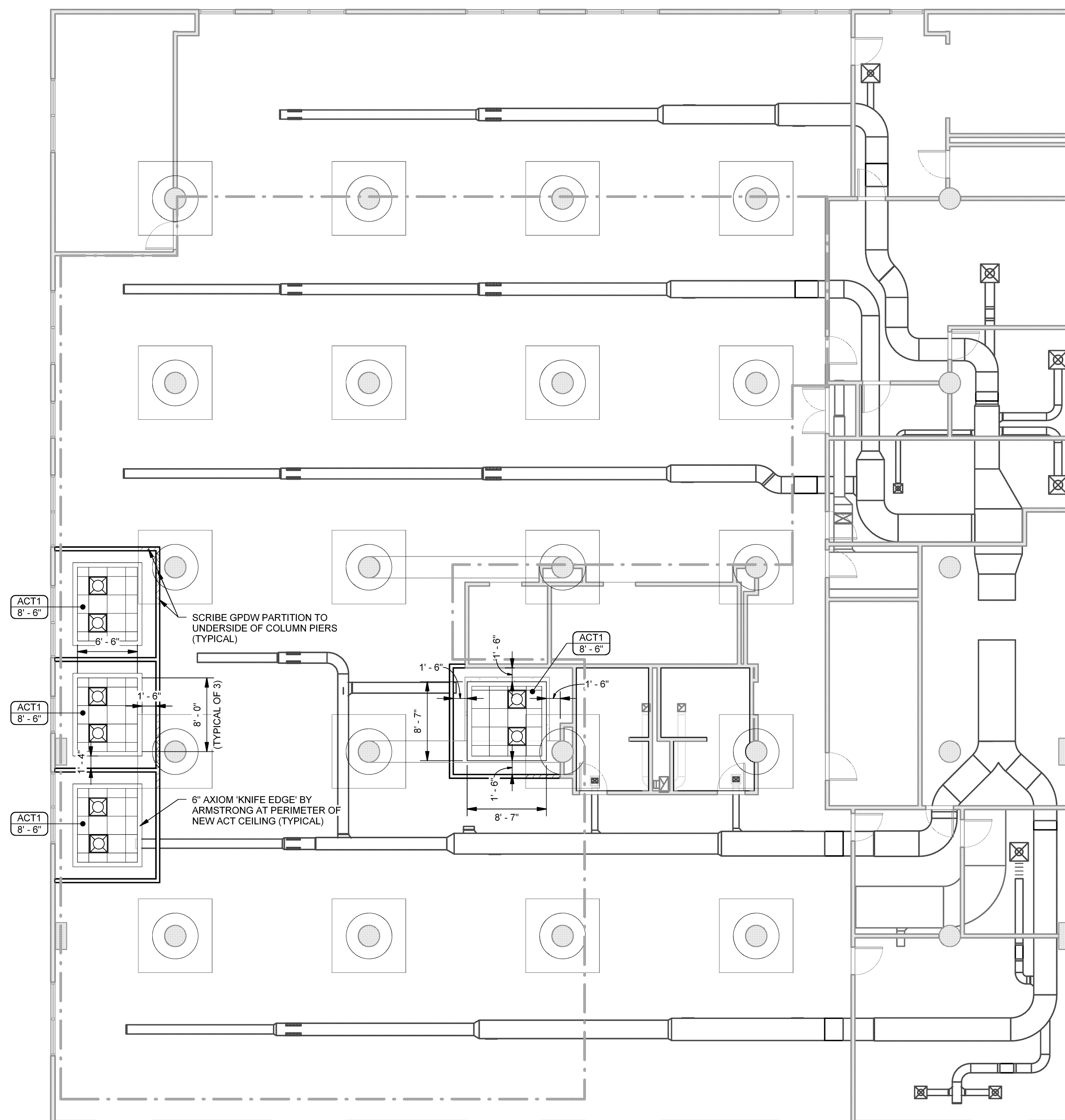
1 THIRD FLOOR CEILING PLAN SCALE: 1/8" = 1'-0"
