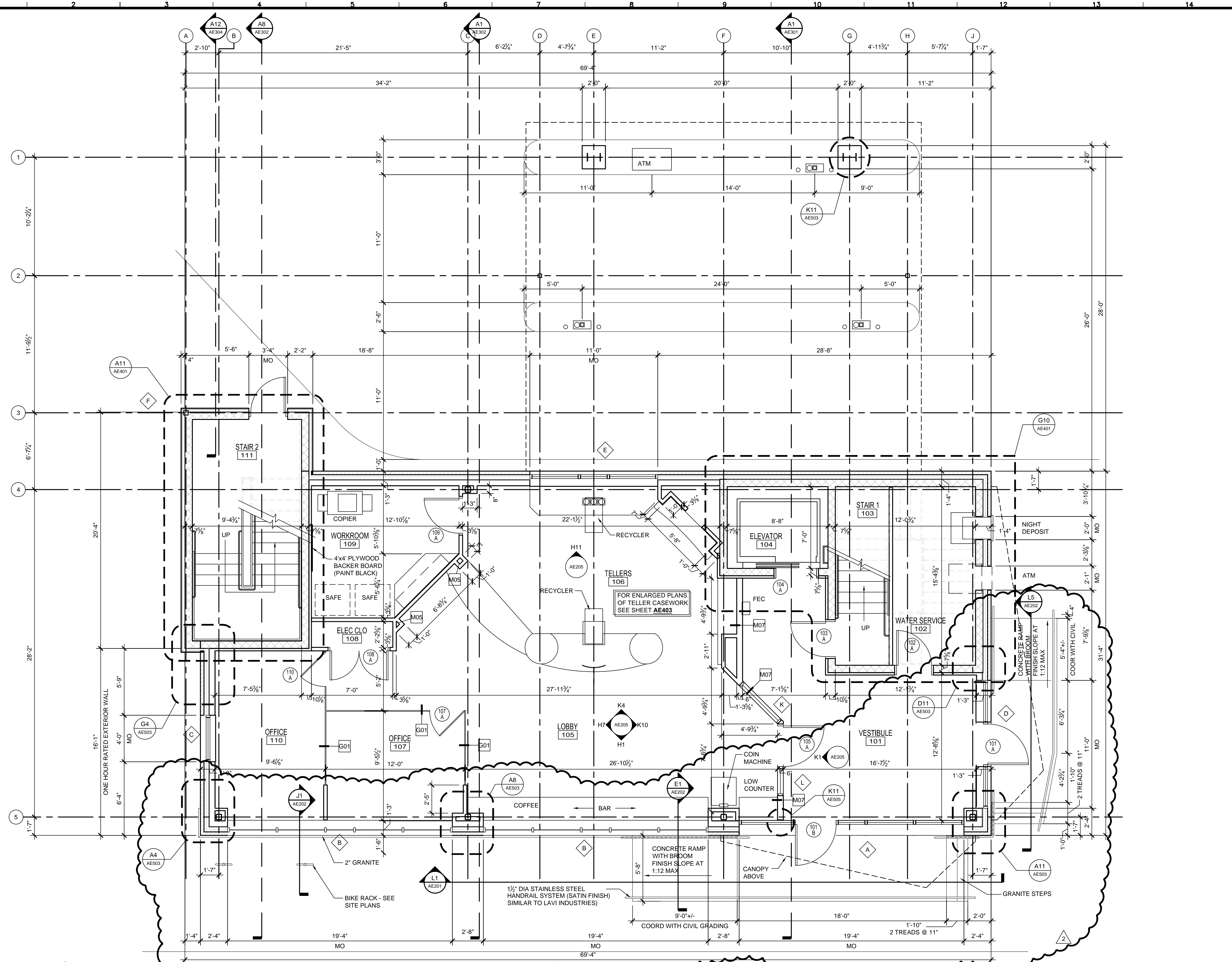
A1 FIRST FLOOR PLAN 1/4" = 1'-0"
