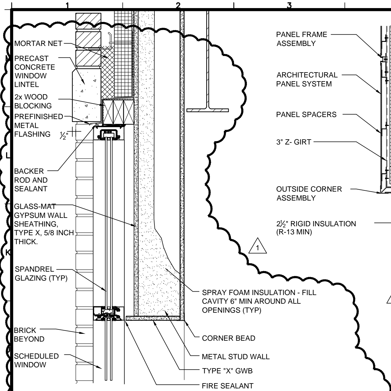
J1 WINDOW HEAD DETAIL @ ALUMINUM FRAME IN 1HR RATED WALL 1/12" = 1'-0"
