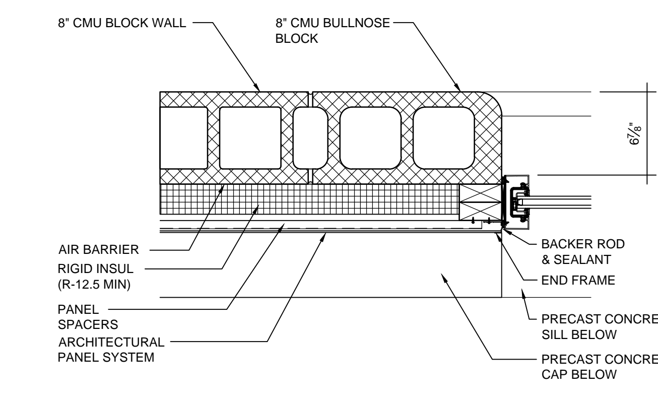
G11 WINDOW JAMB DETAIL @ METAL PANELS & CMU WALL 1/12" = 1'-0"
