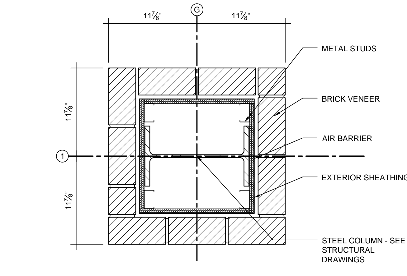
K11 PLAN DETAIL 1/12" = 1'-0"
