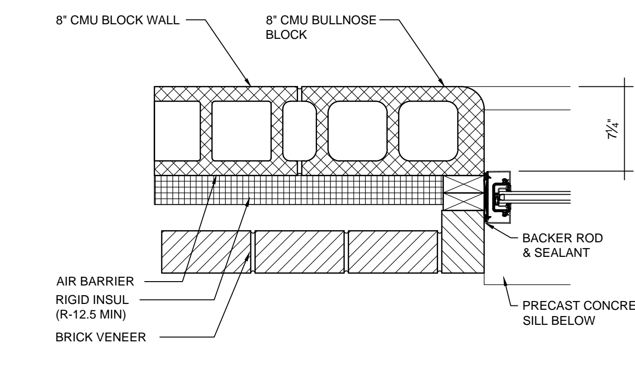
G8 WINDOW JAMB DETAIL @ BRICK VENEER & CMU WALL 1/12" = 1'-0"
