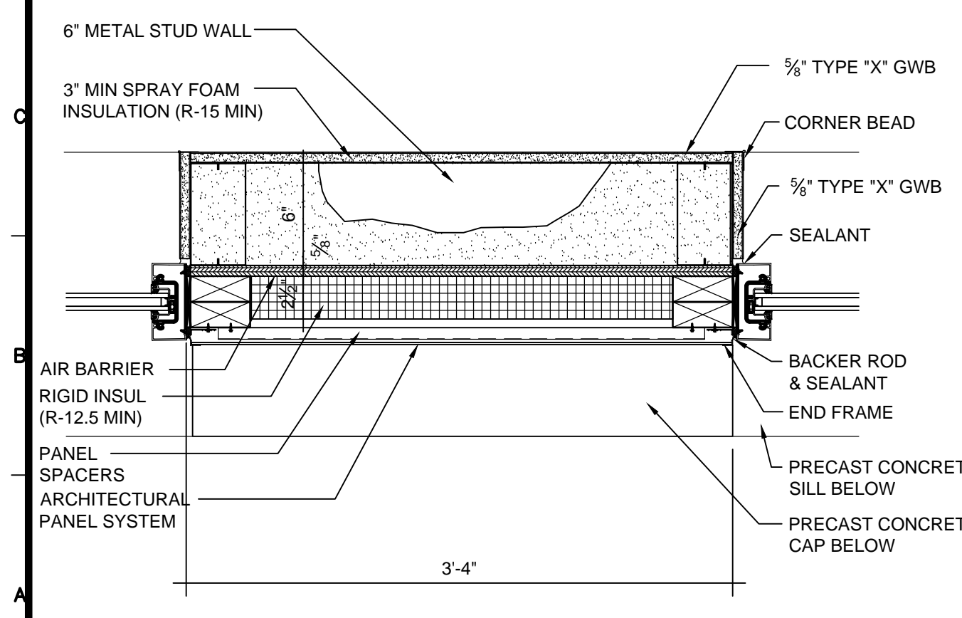
A1 WINDOW JAMB DETAIL @ METAL PANELS 1/12" = 1'-0"
