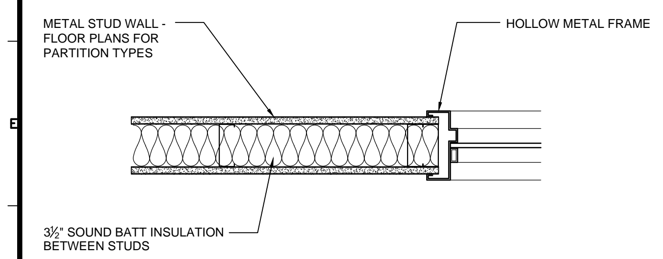
D1 WINDOW JAMB DETAIL @ HOLLOW METAL FRAME 1/12" = 1'-0"
