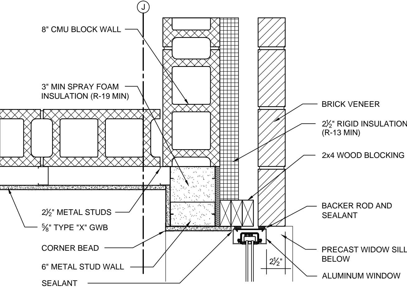
D11 PLAN DETAIL 1/12" = 1'-0"
