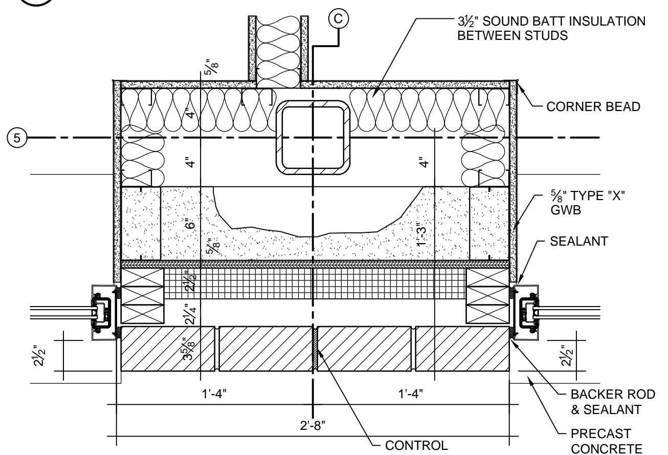
A8 WINDOW JAMB DETAIL @ BRICK VENEER 1/12" = 1'-0"
