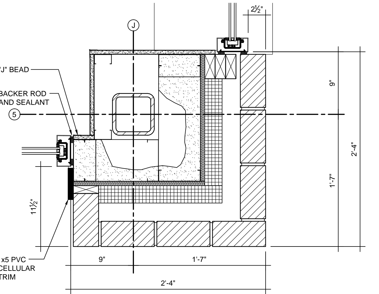
A11 PLAN DETAIL 1/12" = 1'-0"
