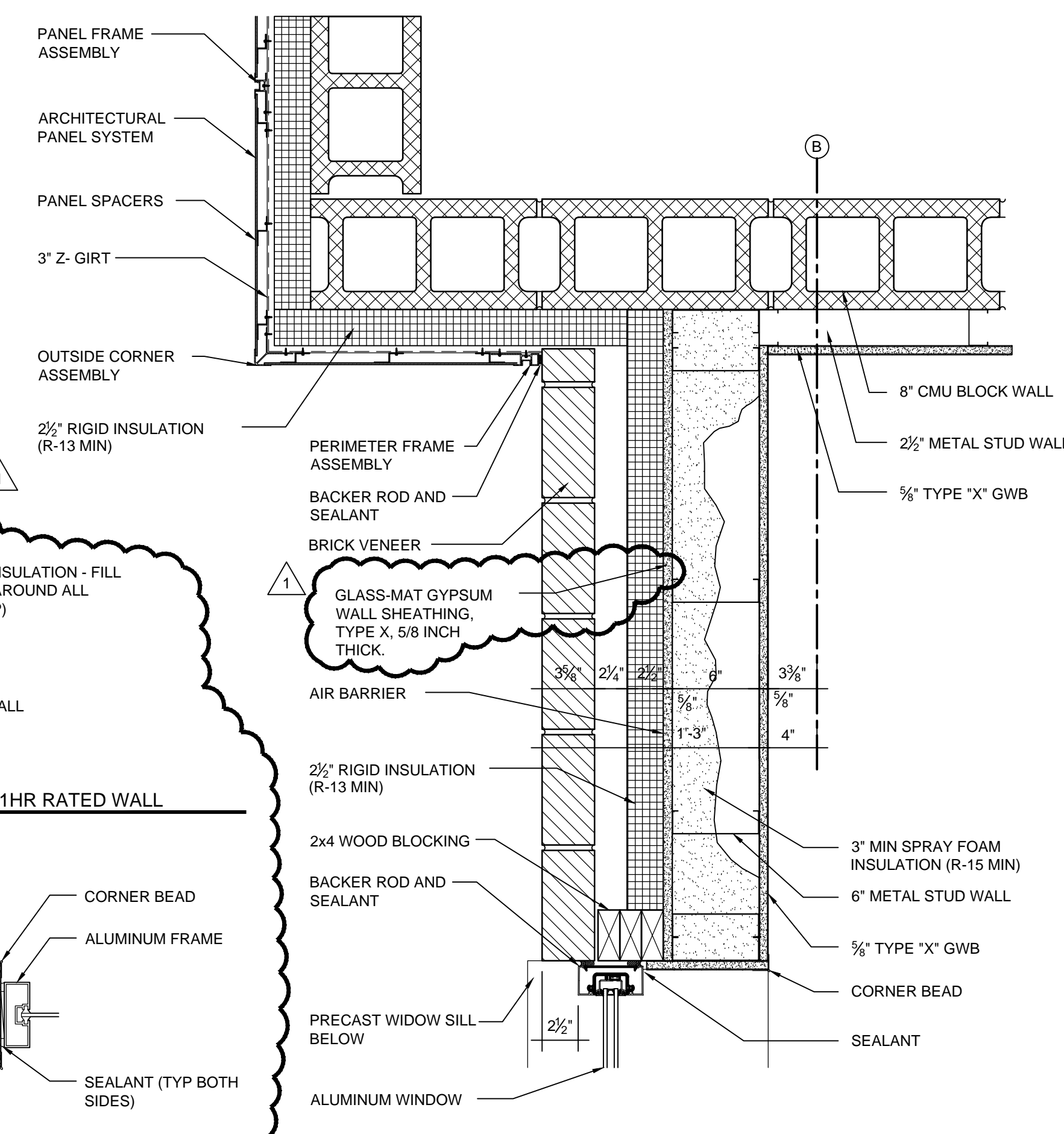
G1 WINDOW JAMB DETAIL @ ALUMINUM FRAME 1/12" = 1'-0"
