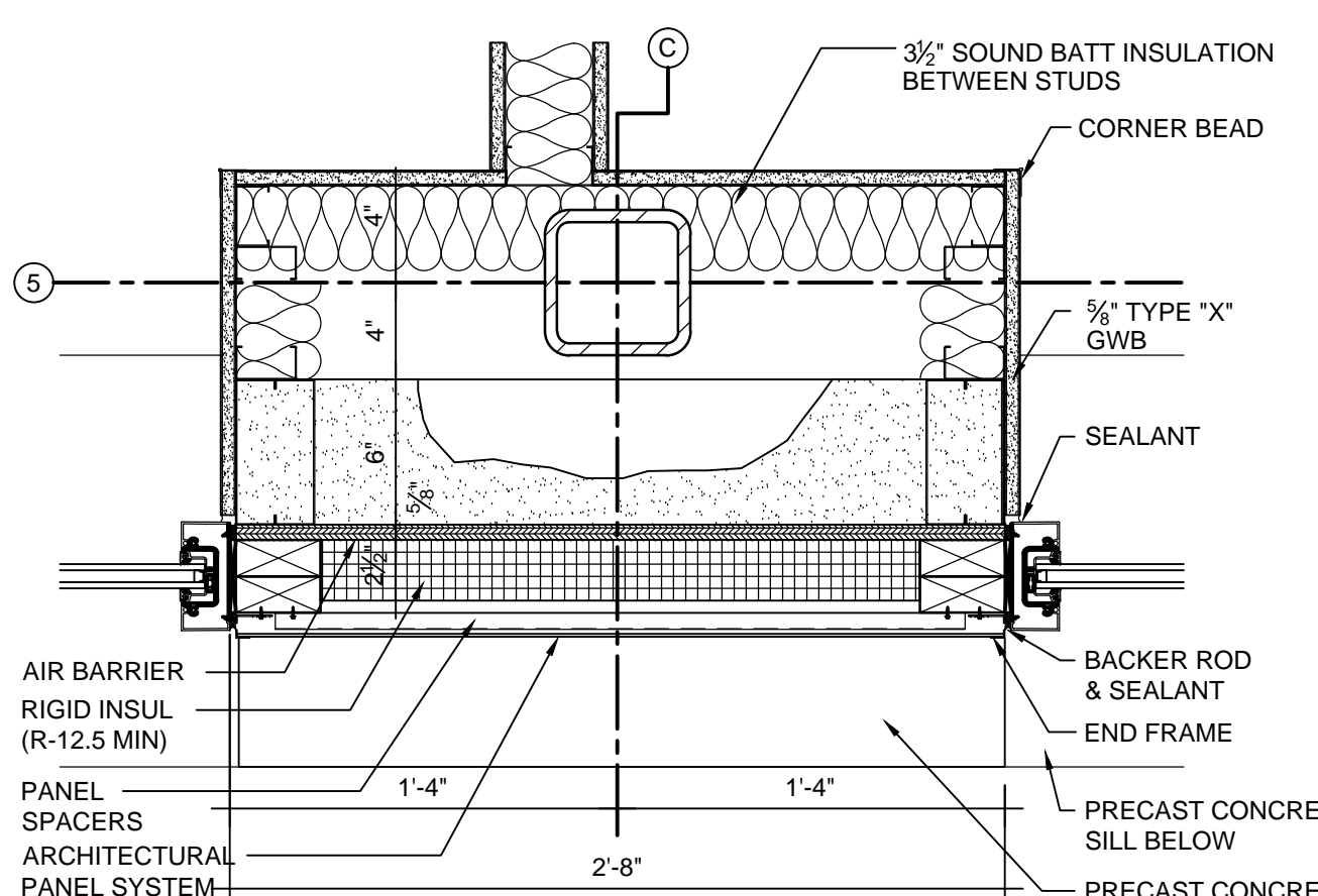
D8 WINDOW JAMB DETAIL @ METAL PANELS 1/12" = 1'-0"
