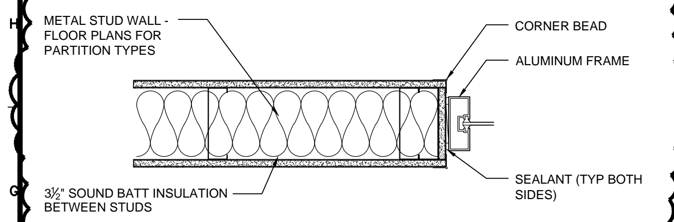
G1 WINDOW JAMB DETAIL @ ALUMINUM FRAME 1/12" = 1'-0"
