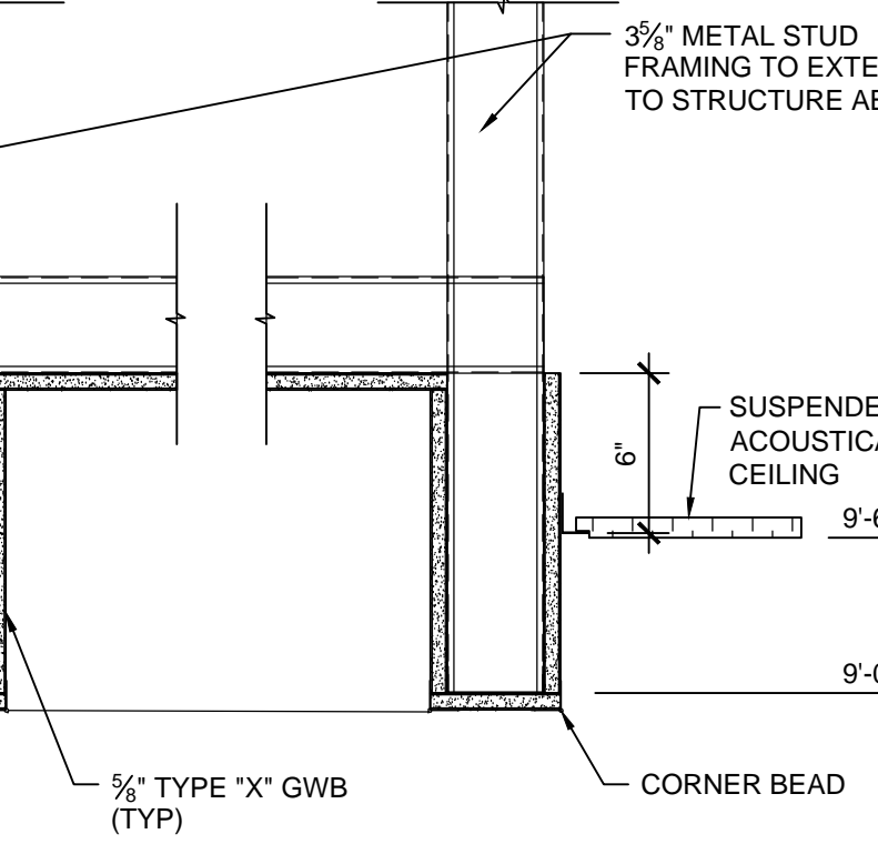
A1 SOFFIT DETAIL @ TELLER LINE 1 1/2" = 1'-0"
