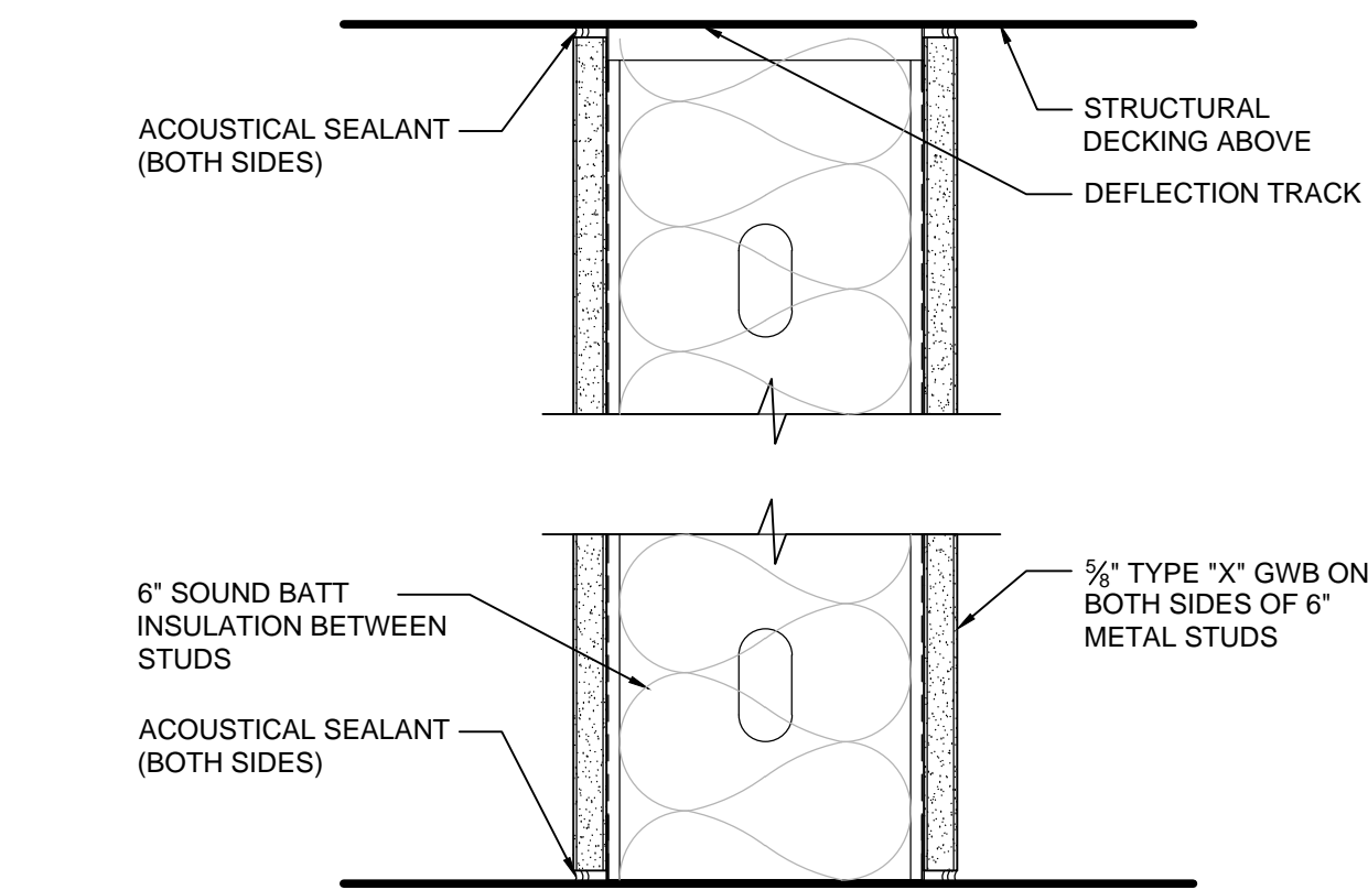
K8 M07 - 6" METAL STUD WALL (SOUND) 3/8" = 1'-0"
