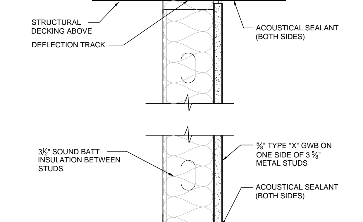
A11 M05 - 3 5/8" METAL STUD CHASE WALL (SOUND) 3/8" = 1'-0"
