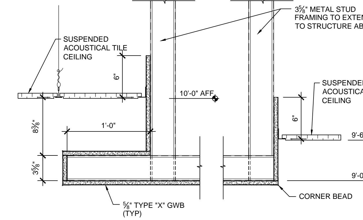
A4 SOFFIT DETAIL @ TELLER LINE 1 1/2" = 1'-0"
