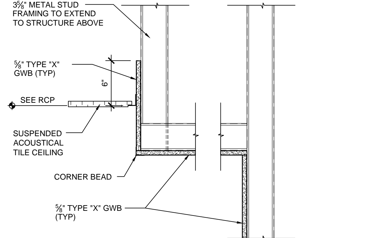
D4 GWB SOFFIT DETAIL 1 1/2" = 1'-0"
