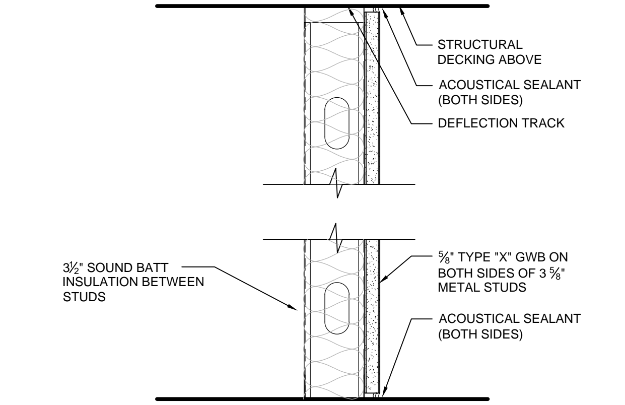
G8 M12 - 2 1/2" METAL STUD CHASE WALL - SOUND 3/8" = 1'-0"
