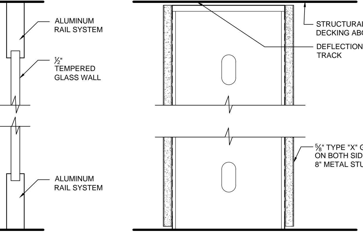
D7 G01 - GLASS WALL 3/8" = 1'-0"
