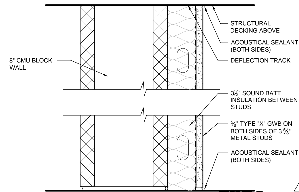
K4 C02 - 8" CMU BLOCK WALL w/ 2 1/2" METAL STUDS 3/8" = 1'-0"
