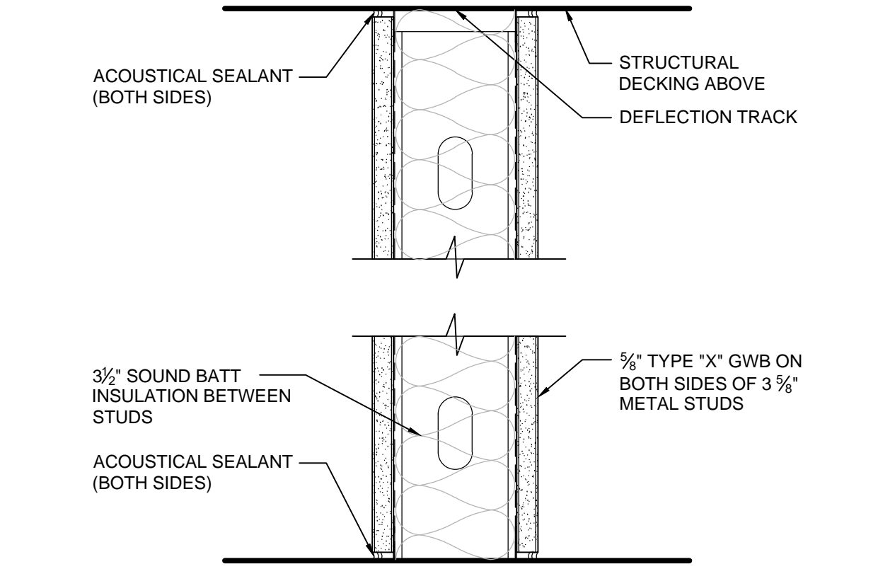
G11 M02 - 3 5/8" METAL STUD WALL (SOUND) 3/8" = 1'-0"
