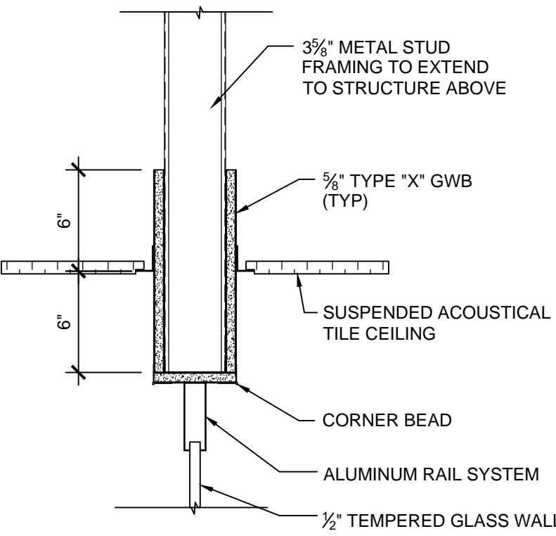
D1 SOFFIT DETAIL @ ALL-GLASS STOREFRONT 1 1/2" = 1'-0"
