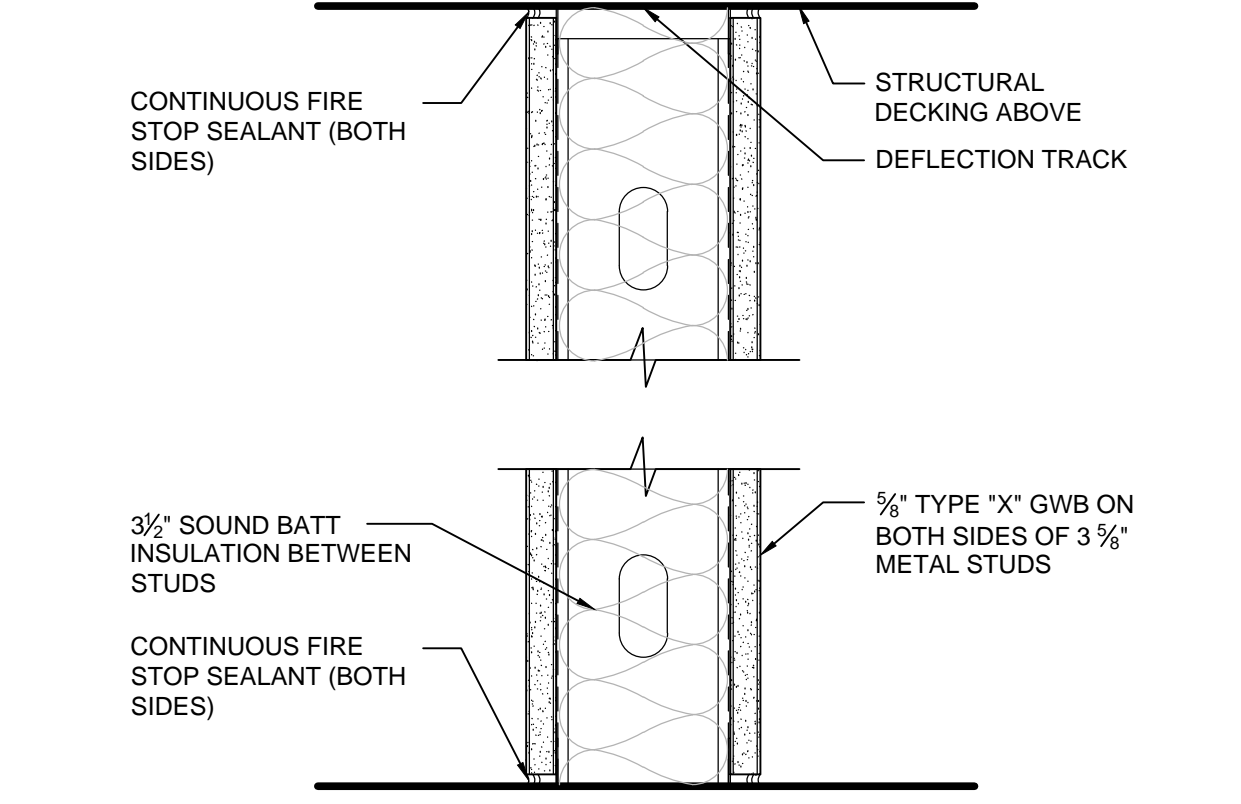
D11 M03 - 3 5/8" METAL STUD WALL (1 HOUR RATED) 3/8" = 1'-0"
