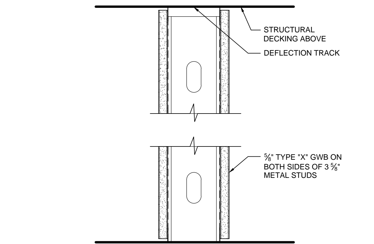
K11 M01 - 3 5/8" METAL STUD WALL 3/8" = 1'-0"
