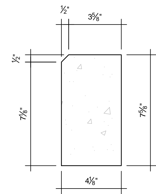
K1 PRECAST CONCRETE LINTEL 3/8" = 1'-0"
