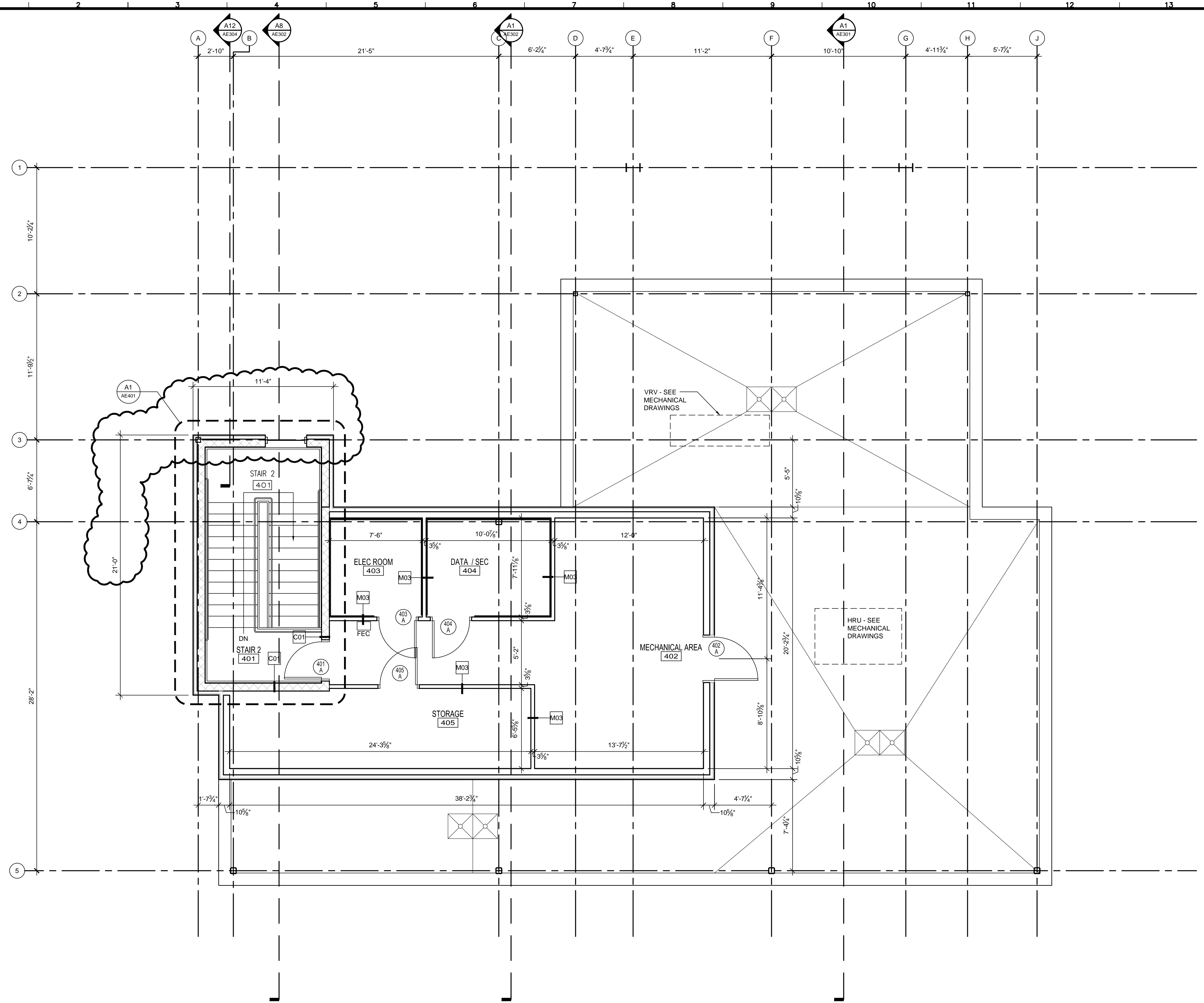
A1 MECHANICAL PENTHOUSE PLAN 1/4" = 1'-0"
