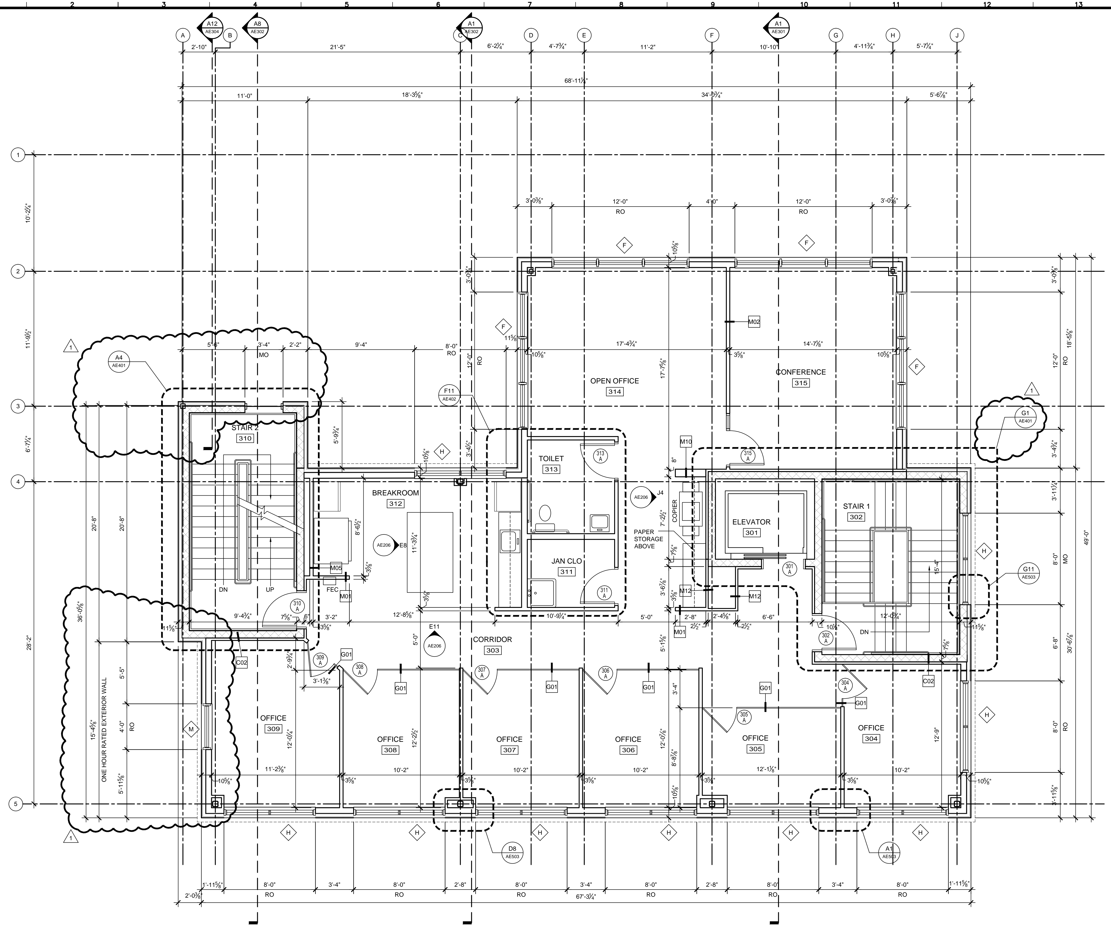
A1 THIRD FLOOR PLAN 1/4" = 1'-0"
