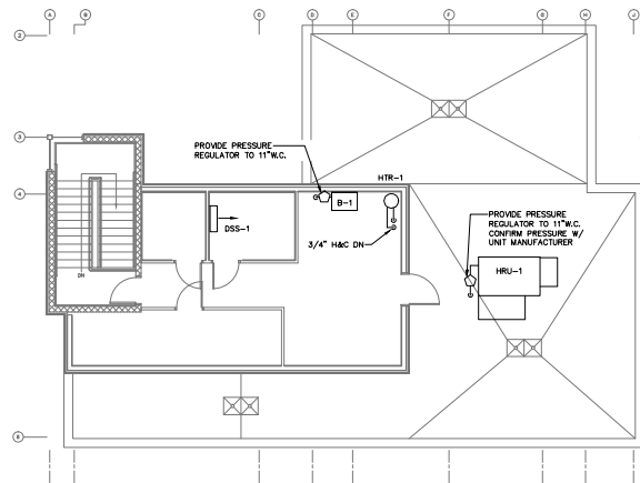
MECHANICAL PENTHOUSE PLAN
