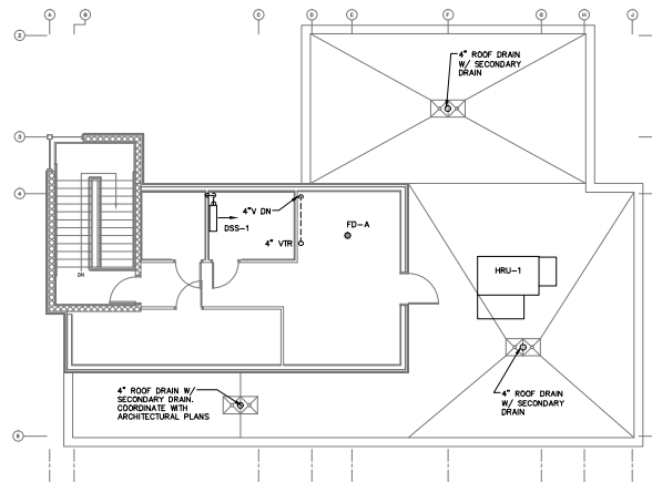
MECHANICAL PENTHOUSE PLAN
