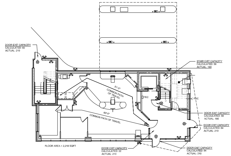
A6 FIRST FLOOR PLAN 38'-0" x 58'-0"
