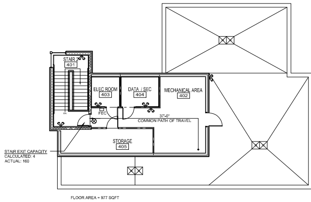
A1 MECHANICAL PENTHOUSE PLAN 18'-0" x 12'-0"
