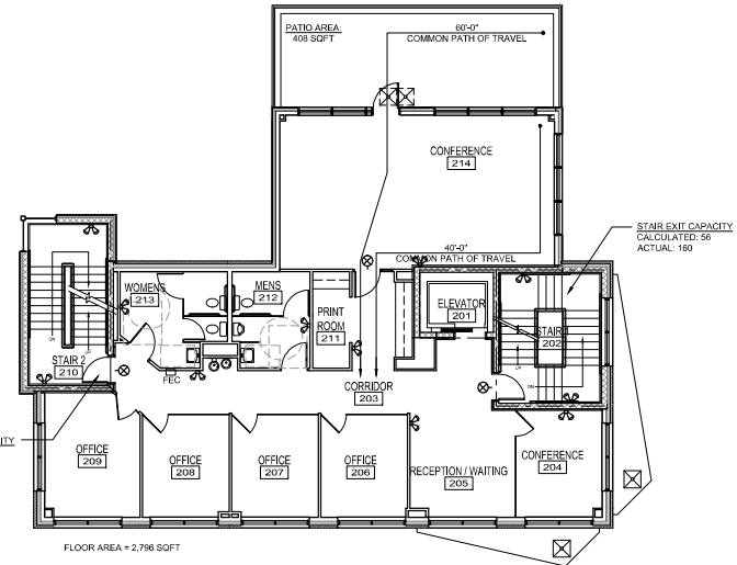
G6 SECOND FLOOR PLAN 38'-0" x 72'-0"
