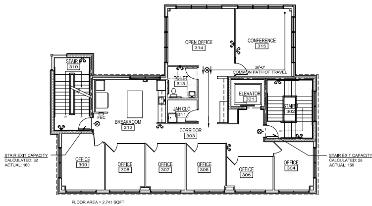
A1 THIRD FLOOR PLAN 18'-0" x 15'-0"
