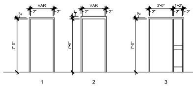
K6 HOLLOW METAL FRAME TYPES
