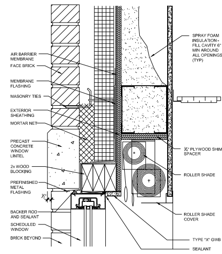
D11 WINDOW HEAD DETAIL @ ROLLED SHADE 1/4" = 1'-0"
