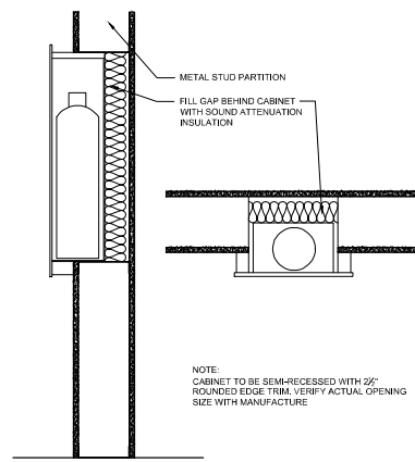
AB SEMI-RECESSED FIRE EXTINGUISHER CABINET 1/4" = 1'-0"
