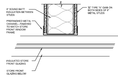
K1 INTERIOR WALL / STORE FRONT INTERSECTION DETAIL 1/4" = 1'-0"
