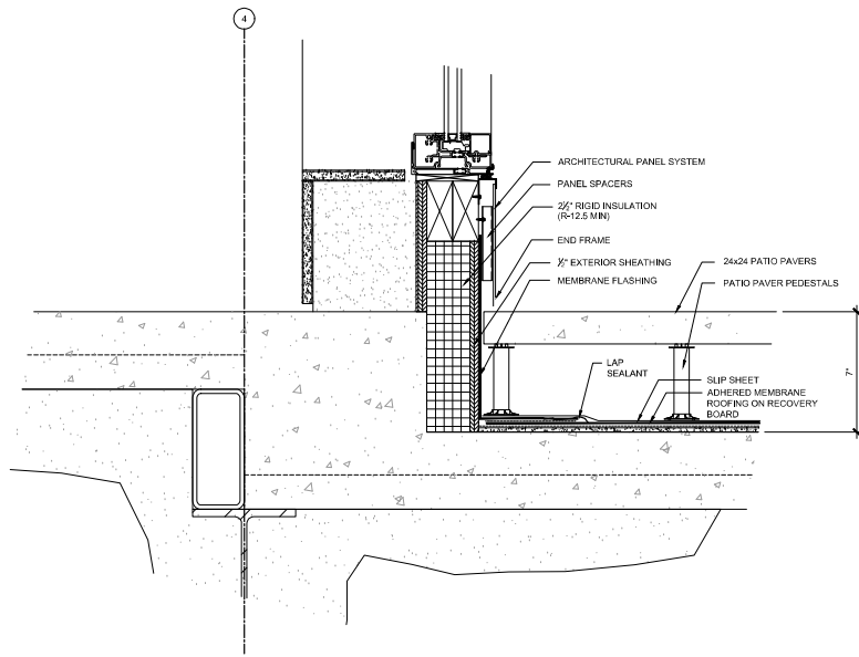
G4 PATIO ROOF / WALL DETAIL 1/4" = 1'-0"
