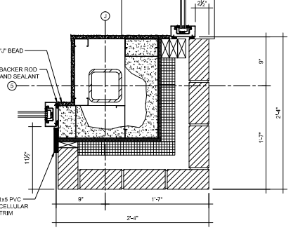
A11 PLAN DETAIL 1:12 = 1:2"
