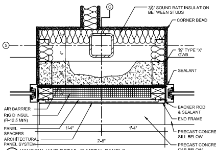
D8 WINDOW JAMB DETAIL @ METAL PANELS 1:12 = 1:2"
