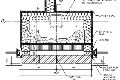
A8 WINDOW JAMB DETAIL @ BRICK VENEER 1:12 = 1:2"
