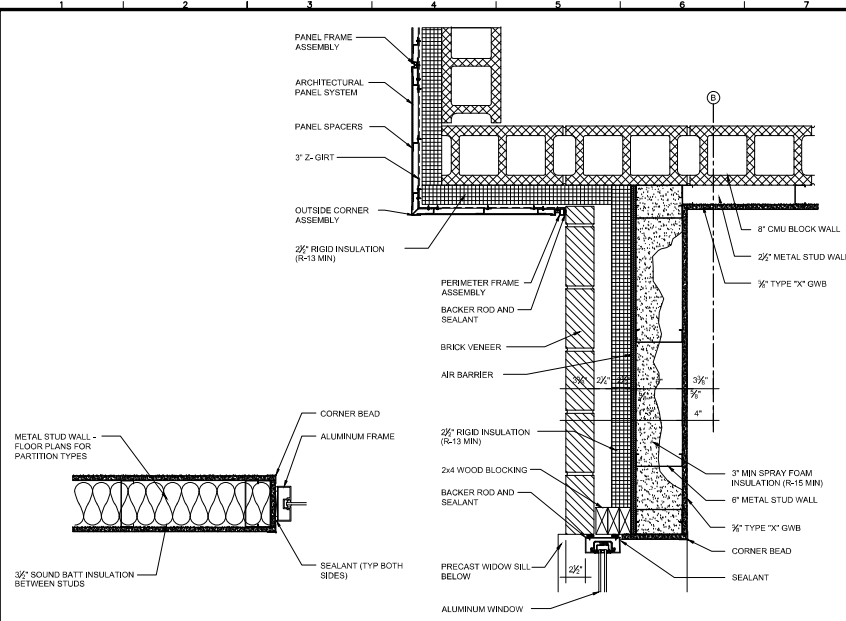
G4 WINDOW JAMB DETAIL @ ALUMINUM FRAME 1:12 = 1:2"
