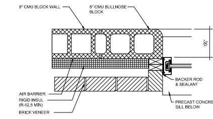
G8 WINDOW JAMB DETAIL @ BRICK VENEER & CMU WALL 1:12 = 1:2"
