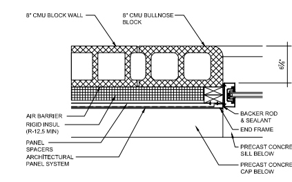
G11 WINDOW JAMB DETAIL @ METAL PANELS & CMU WALL 1:12 = 1:2"
