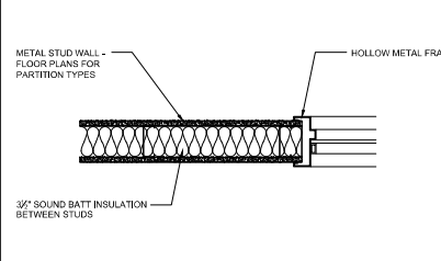
D1 WINDOW JAMB DETAIL @ HOLLOW METAL FRAME 1:12 = 1:2"
