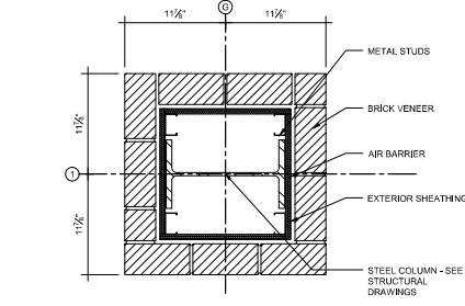
K11 PLAN DETAIL 1:12 = 1:2"
