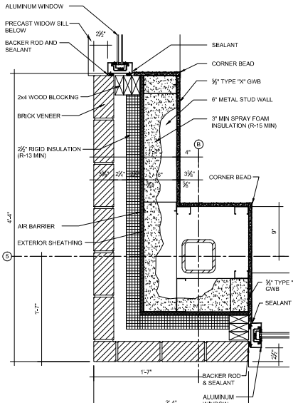
A4 PLAN DETAIL 1:12 = 1:2"
