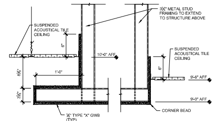
A4 SOFFIT DETAIL @ TELLER LINE 1/2" x 1/2"
