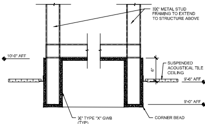
A1 SOFFIT DETAIL @ TELLER LINE 1/2" x 1/2"
