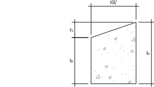
G4 PRECAST CONCRETE CAP 1/2" x 1/2"
