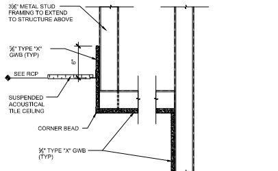
D4 GWB SOFFIT DETAIL 1/2" x 1/2"
