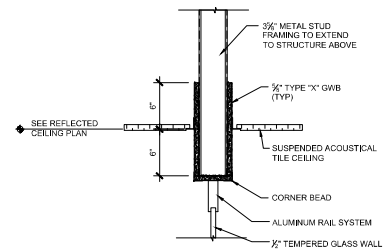
D1 SOFFIT DETAIL @ ALL-GLASS STOREFRONT 1/2" x 1/2"
