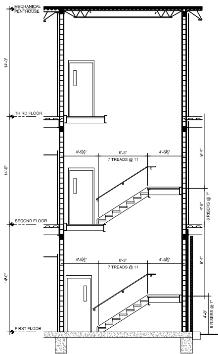
A1 SECTION THRU STAIR #1 1/2\"/>
