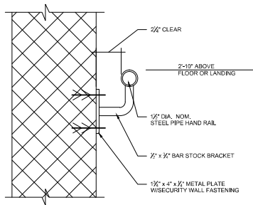
H4 SECTION THRU HANDRAIL 1/2\"/>
