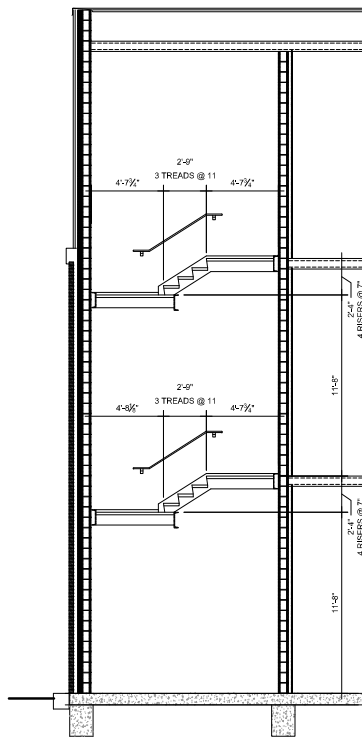
H11 METAL HANDRAIL @ TOP OF STAIR RUN 1 1/2\"/>
