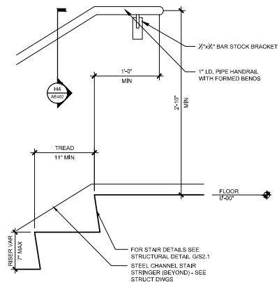
H11 METAL HANDRAIL @ TOP OF STAIR RUN 1 1/2\"/>
