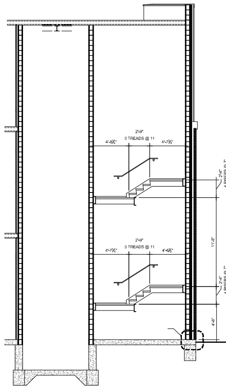
A5 SECTION THRU STAIR #1 1/2\"/>
