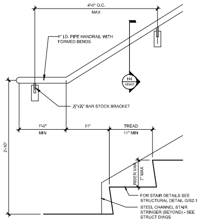
H8 METAL HANDRAIL @ BOTTOM OF STAIR RUN 1 1/2\"/>
