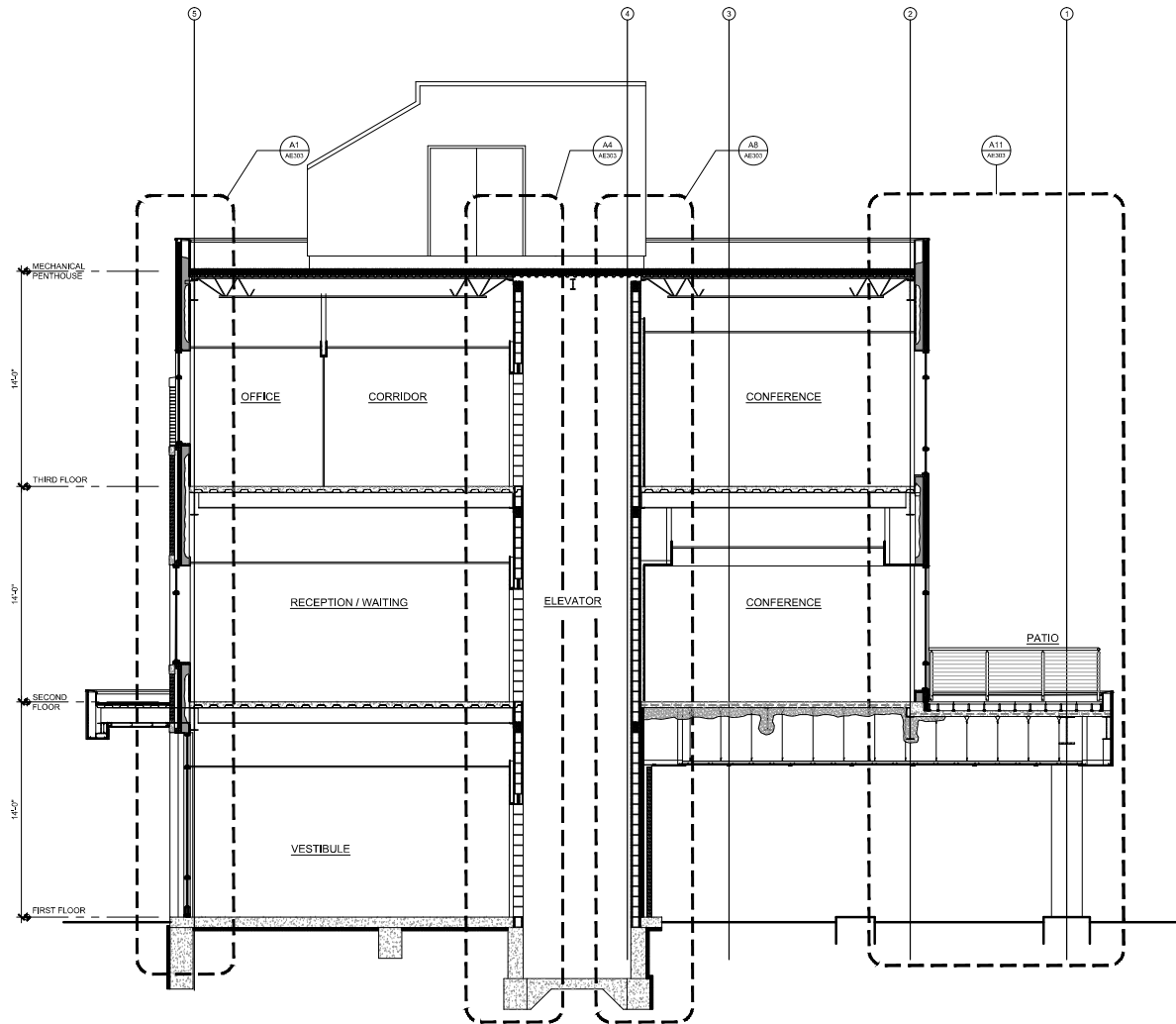
A1 BUILDING SECTION 14'-0"
