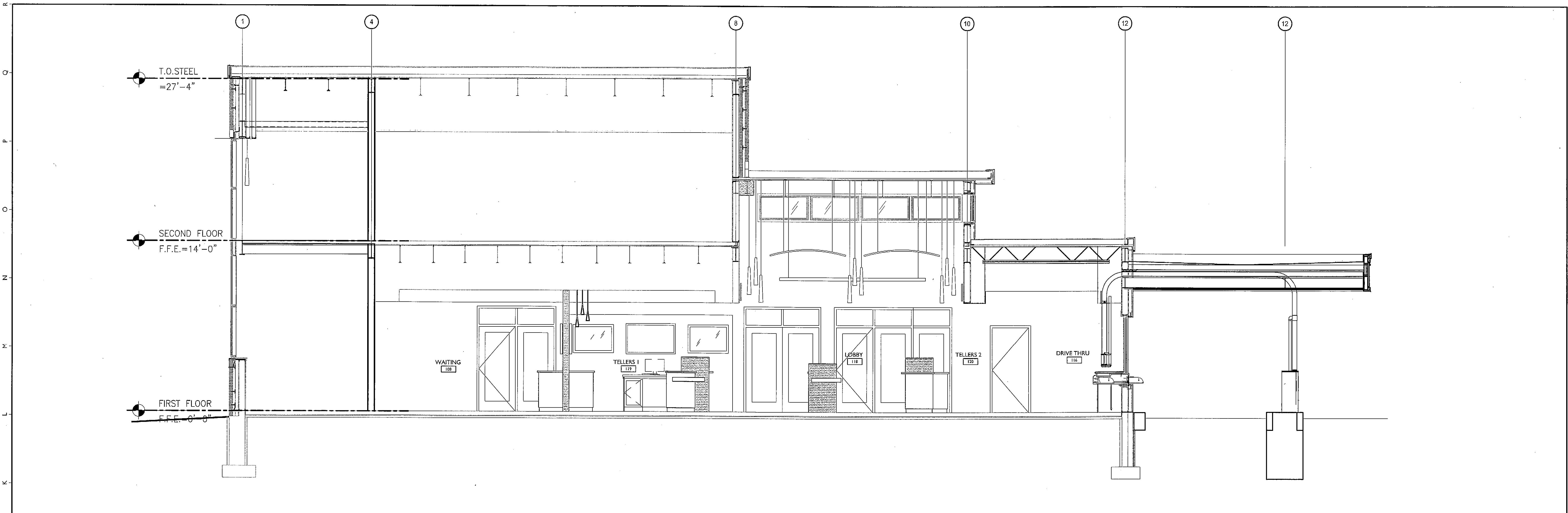
J I BUILDING SECTION
