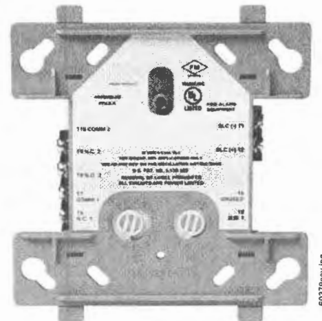
NC-100R(A)
