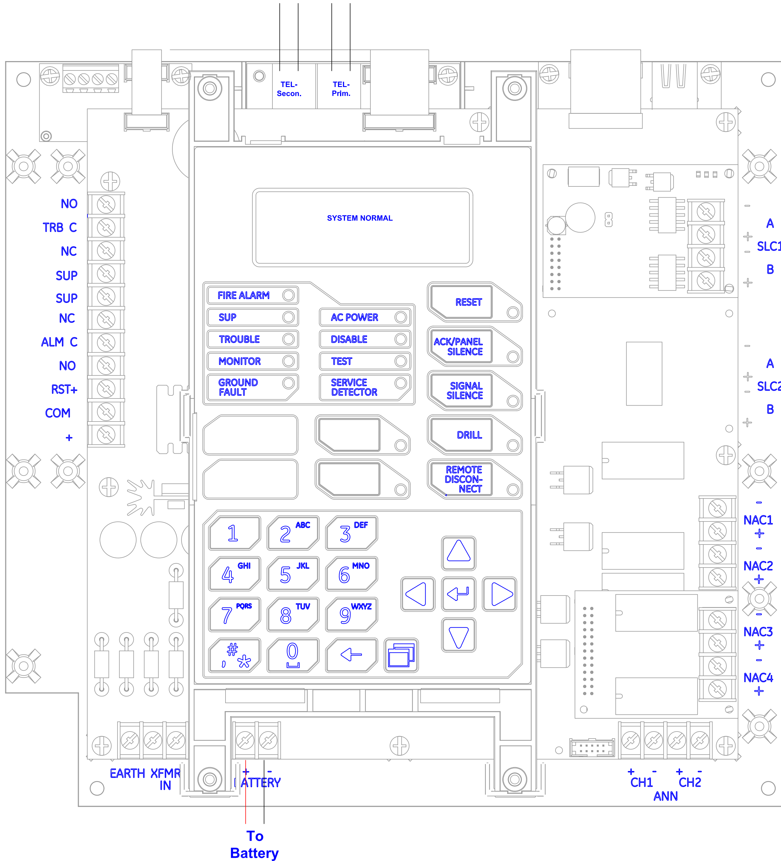
iO64 EST Addressable Panel Panel Wiring Diagram
