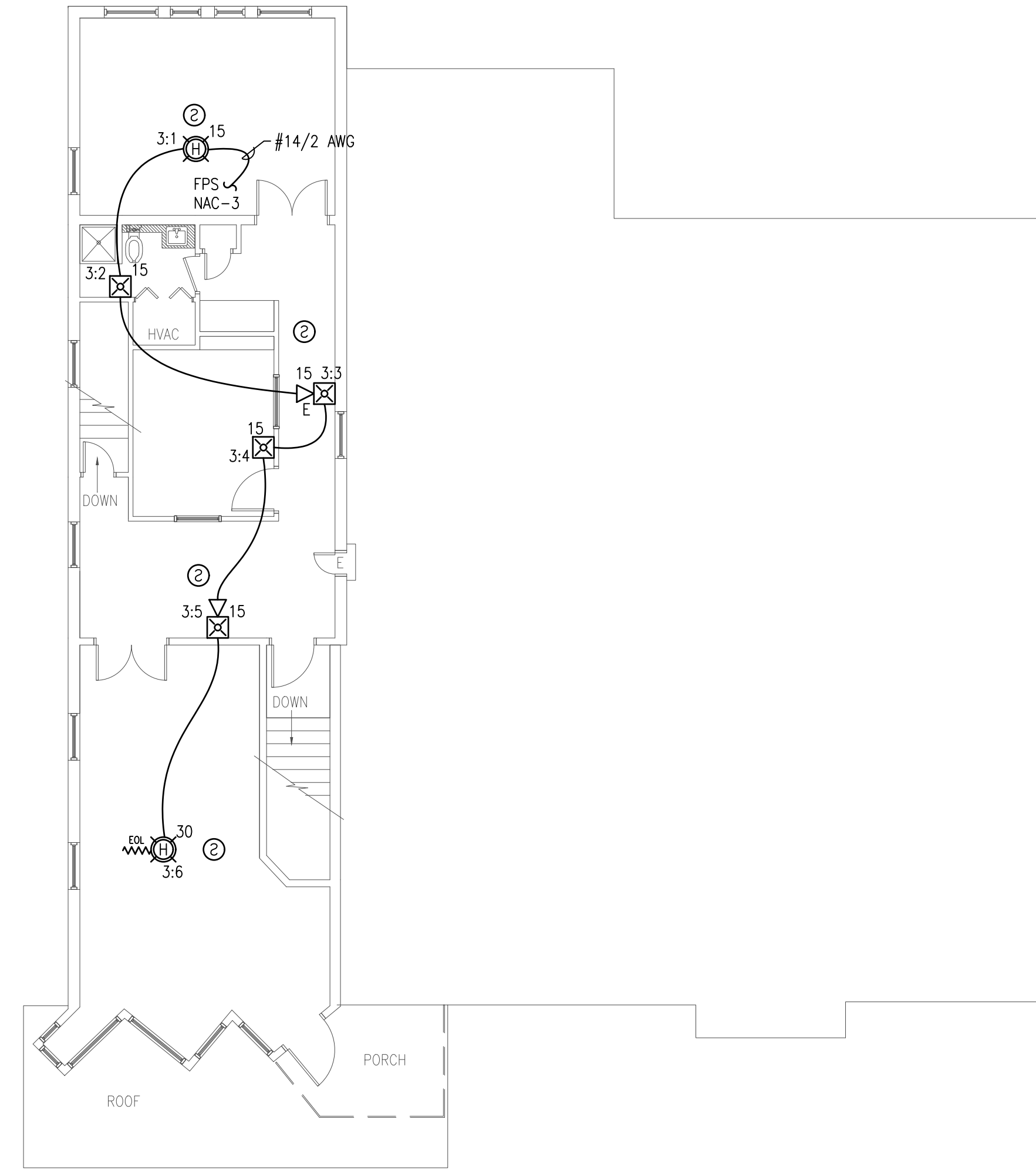
LEVEL 2 FIRE ALARM PLAN SCALE: 1/8"=1'-0"
