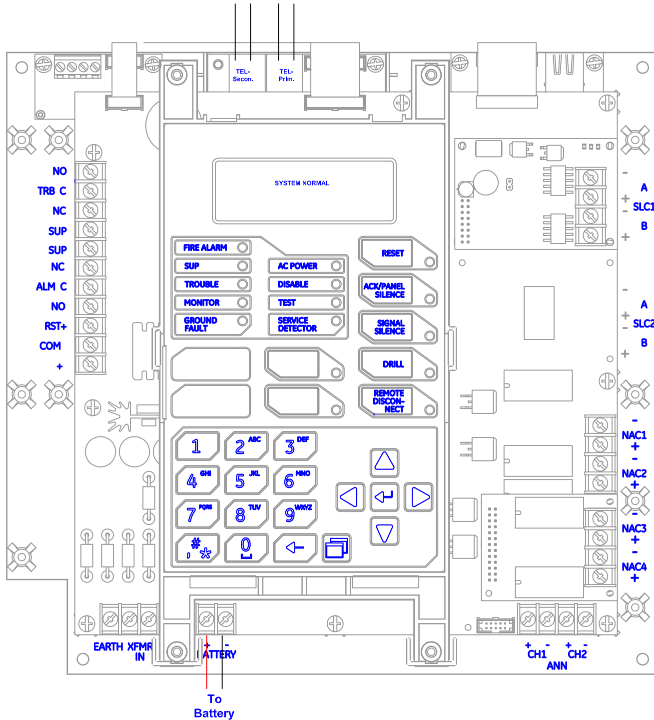
i064 EST Addressable Panel Panel Wiring Diagram
