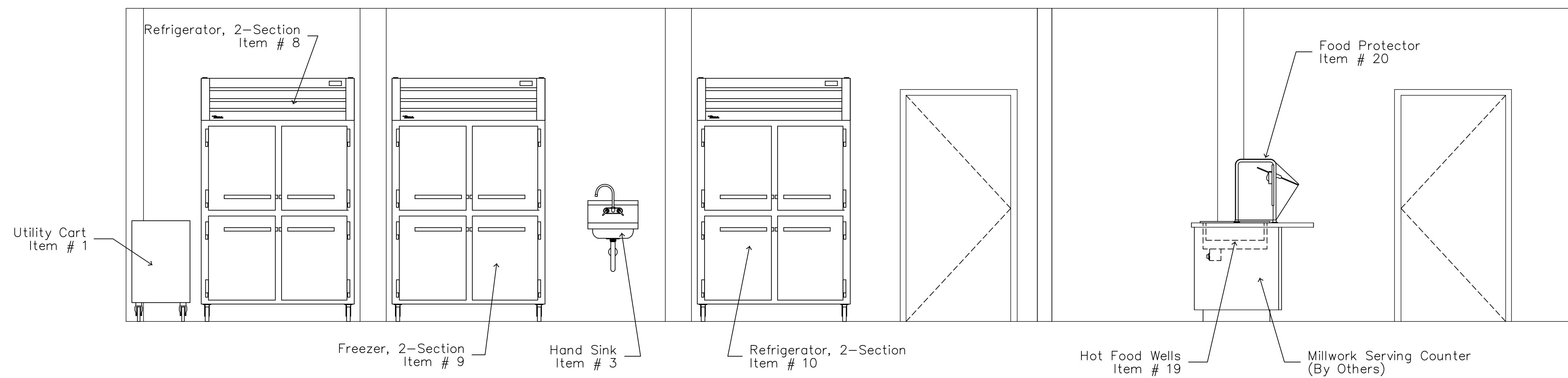
Kitchen North Wall Elevation
