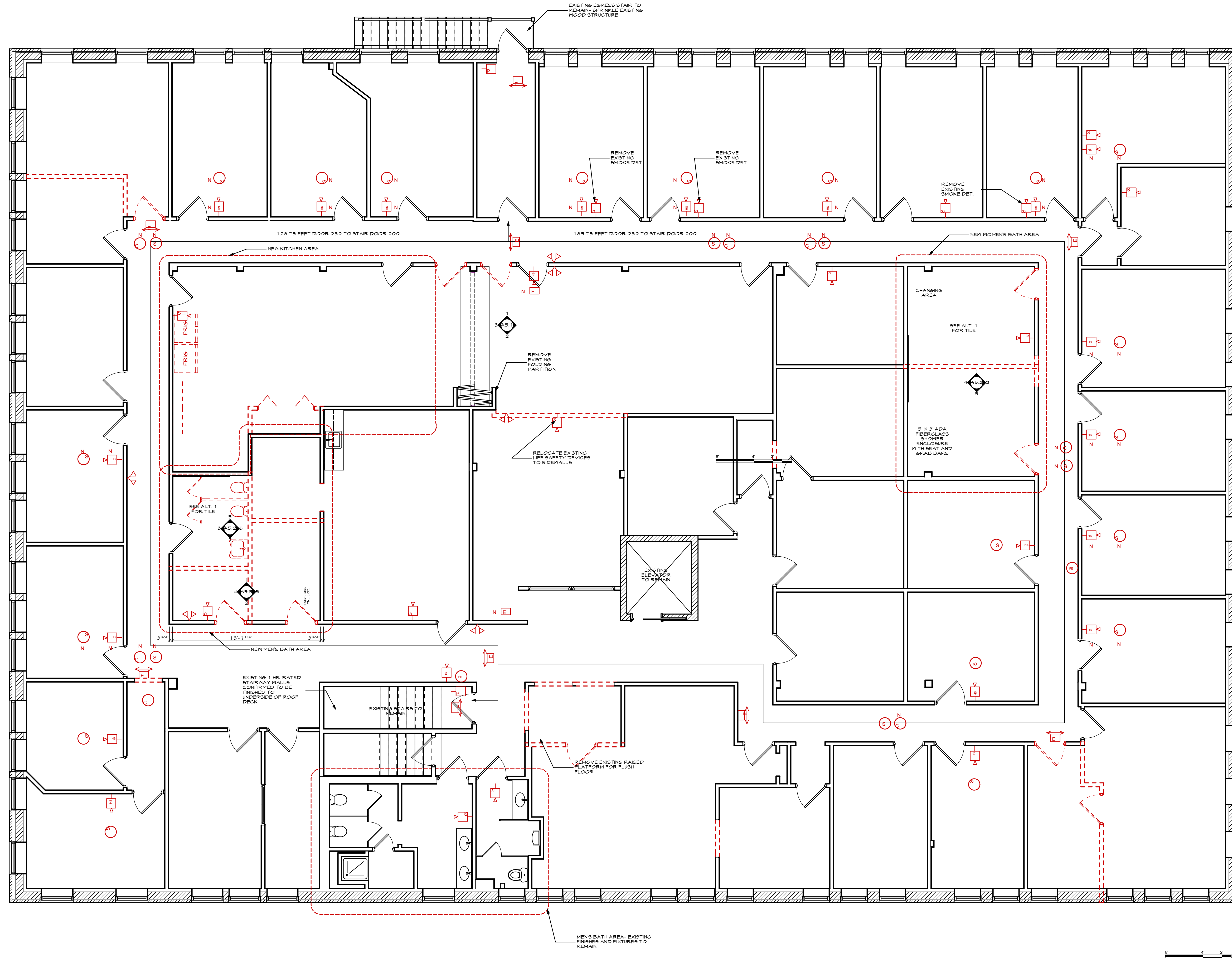
1 SECOND FLOOR DEMO PLAN D1.2 SCALE: 3/16" = 1'-0"
