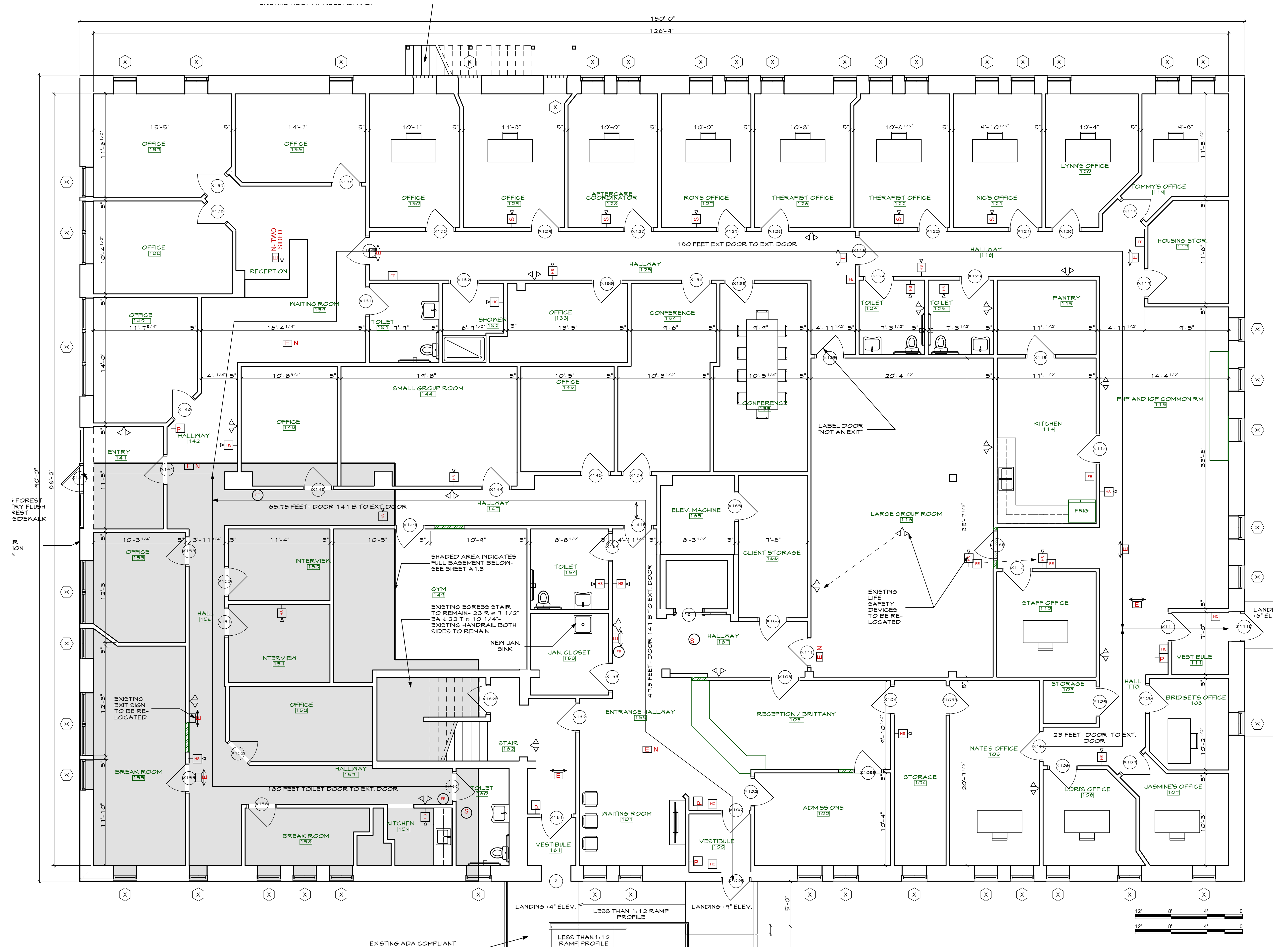
1 FIRST FLOOR PLAN SCALE: 3/16" = 1'-0"
