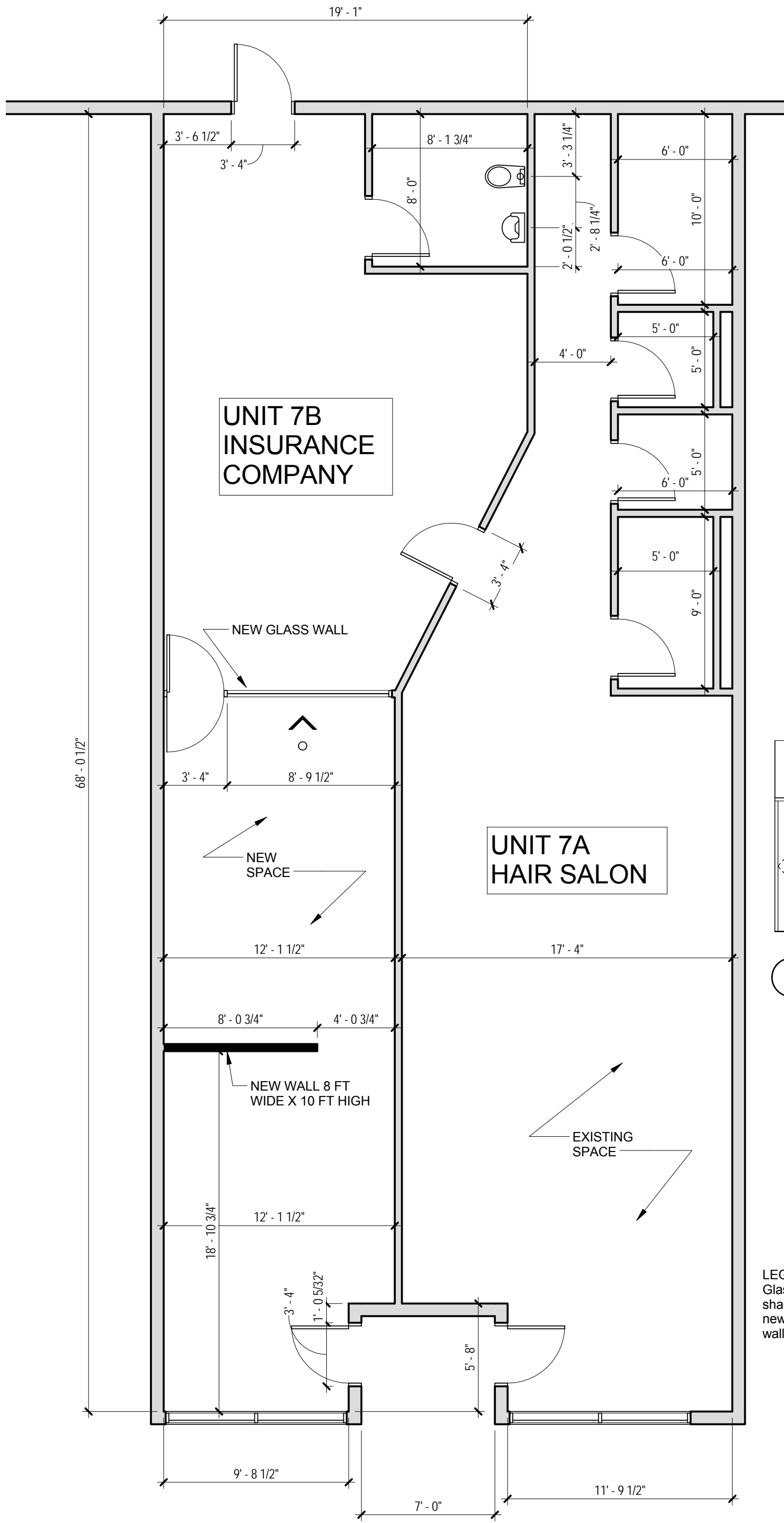
1 FLOOR PLAN FOR DIMENSIONS AND MARKING 3/16" = 1'-0"
