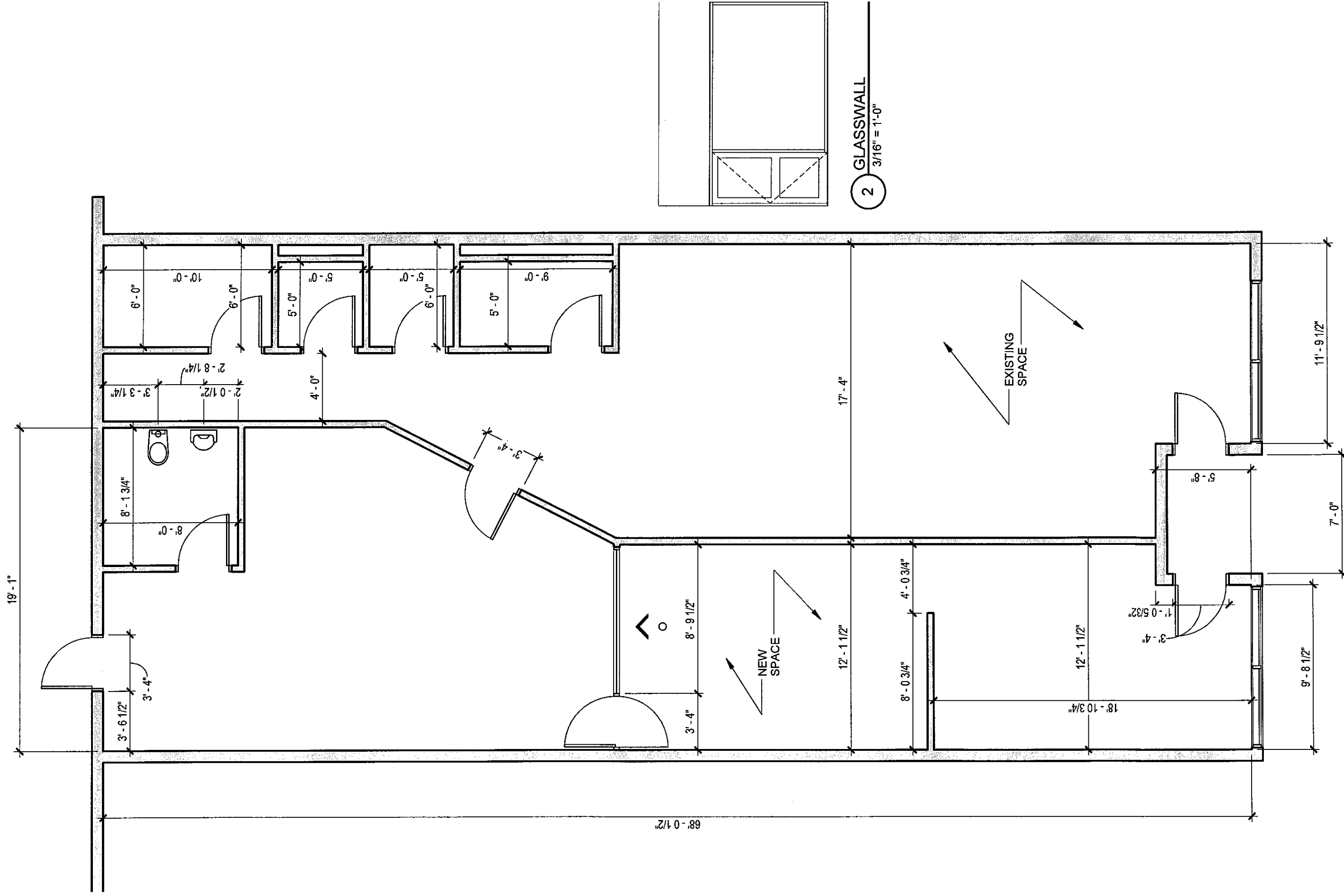
FLOOR PLAN FOR DIMENSIONS AND MARKING
