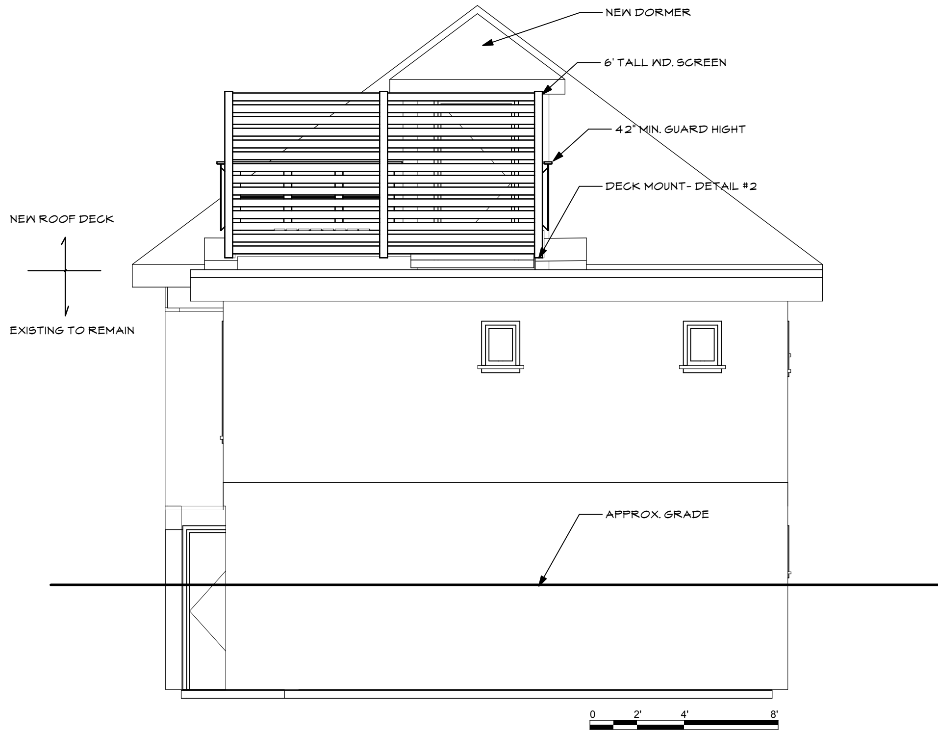
1 West Elevation A2.2 SCALE: 1/4" = 1'-0"
