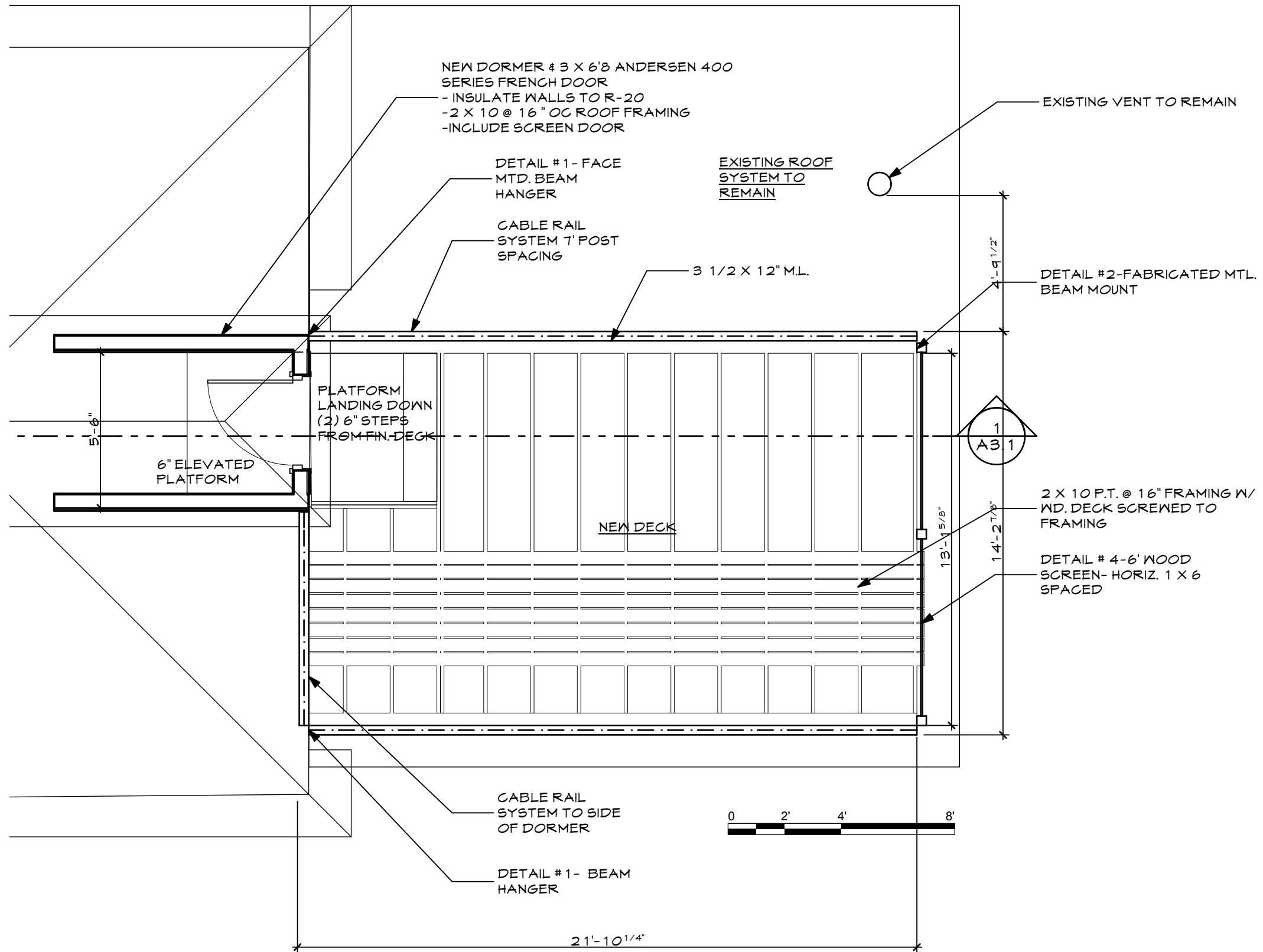
1 New Deck Plan A1.3 SCALE: 1/4" = 1'-0"
