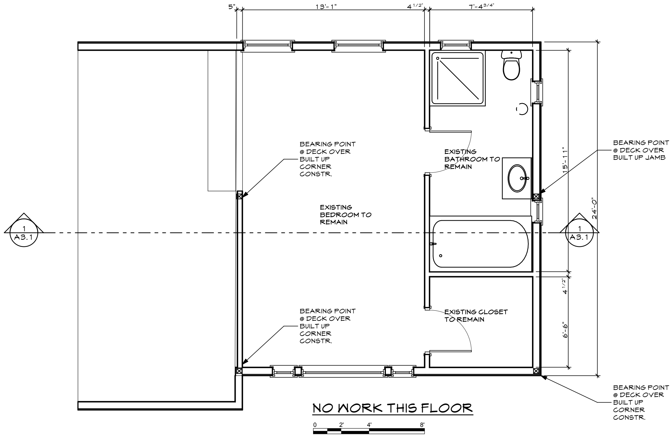
1 Exist. Flr. 1 Plan A1.2 SCALE: 1/4" = 1'-0"
