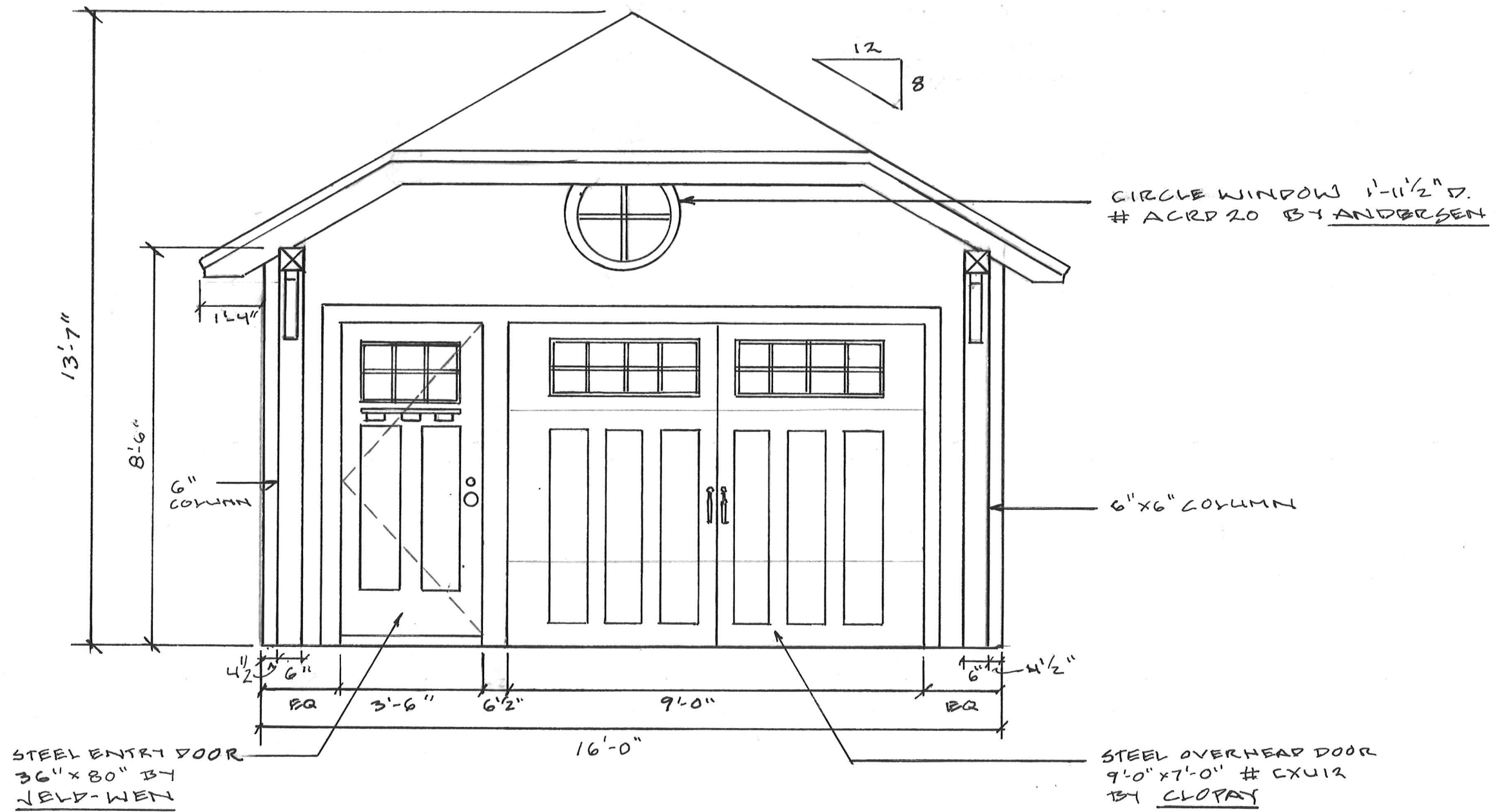
③ FRONT ELEVATION - GARAGE @ 95 DEERFIELD ROAD, PORTLAND ME SCALE: 3/8" = 1'-0"
