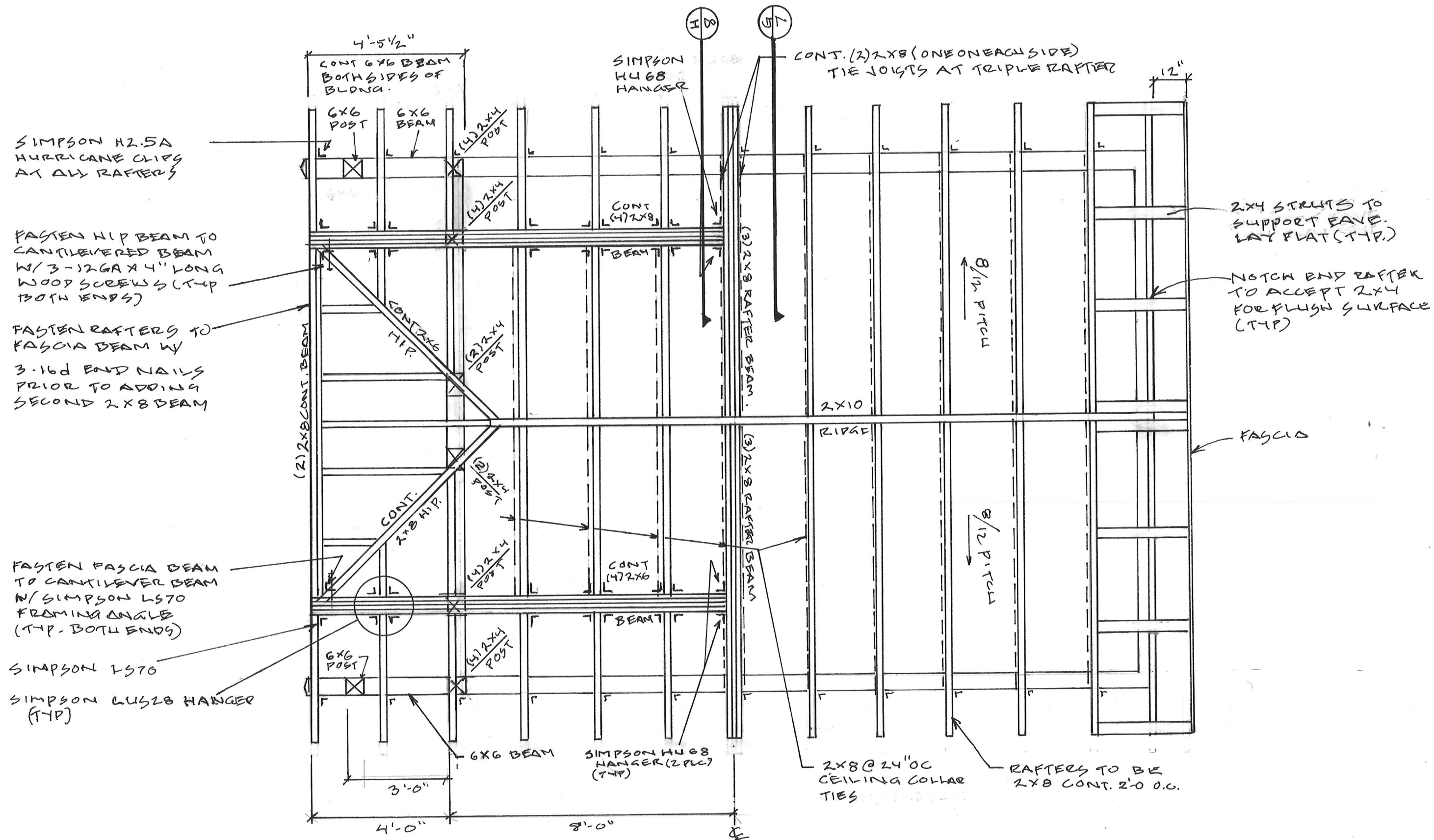
F ROOF FRAMING PLAN SCALE: 3/8" = 1'-0"
