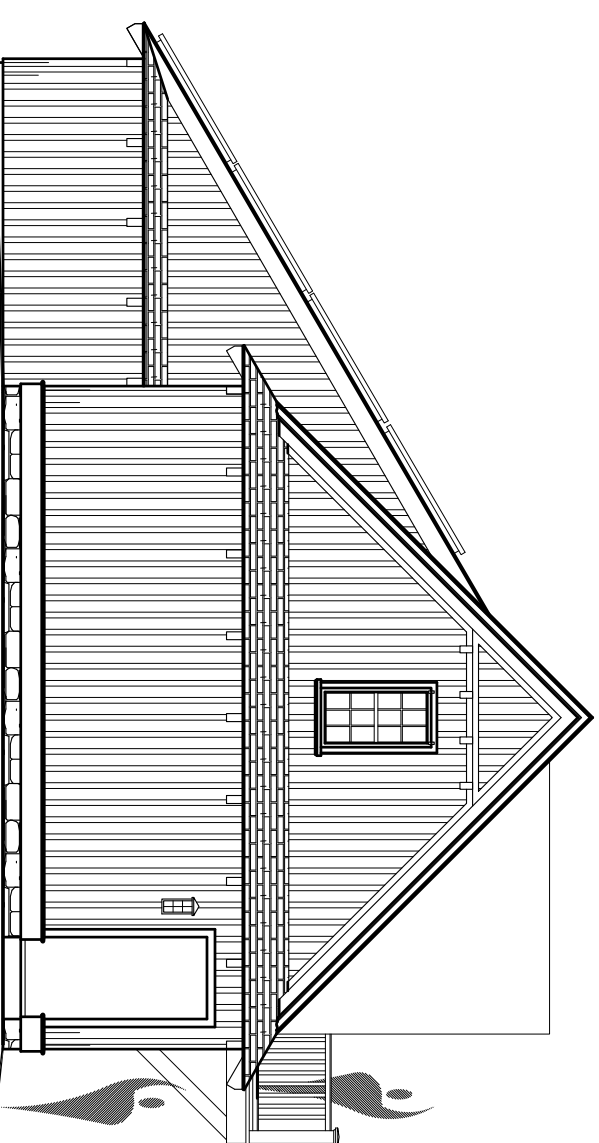
Building #4 East Elevation
