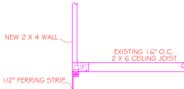
NEW WALL ADDITION DETAIL
