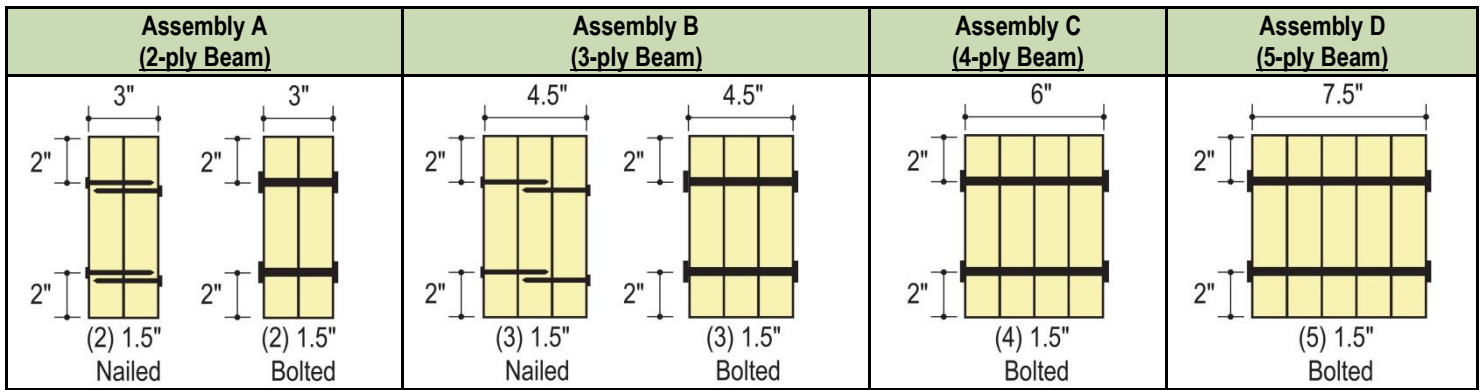
Figures 1A-1D: Connection Requirements for Multiple Member Side-Loaded Beams
