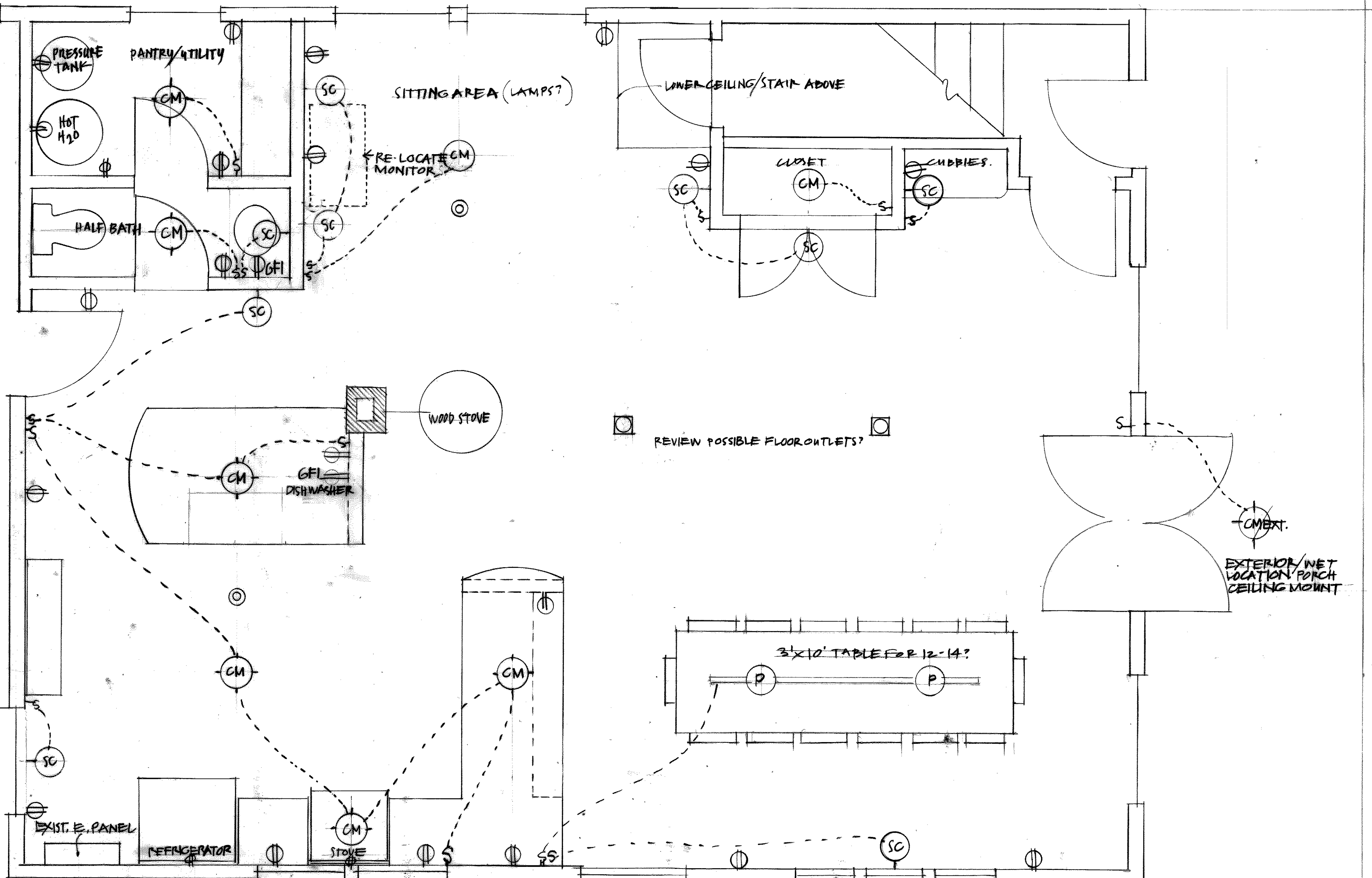
MACVANE HOUSE : ELECTRICAL SCHEMATIC PLAN 1/2" = 1'-0" SCALE 5 NOV. 2015 REDHOUSE ARCHITECTS
