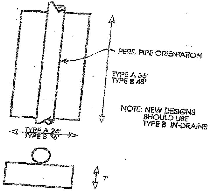
STANDARD IN-DRAIN MODULE
