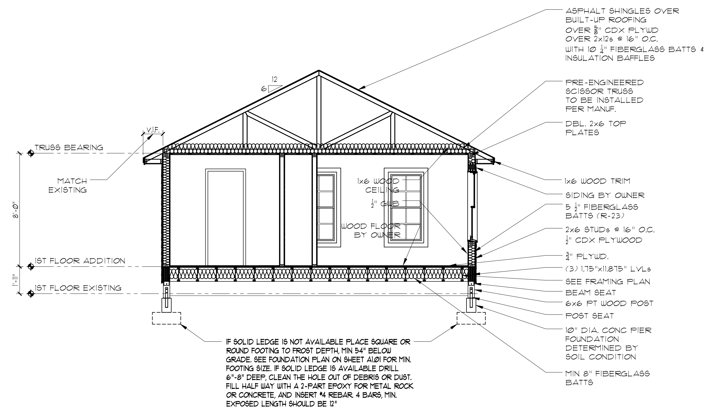
BUILDING SECTION 'C' SCALE: 1/4"=1'-0"
