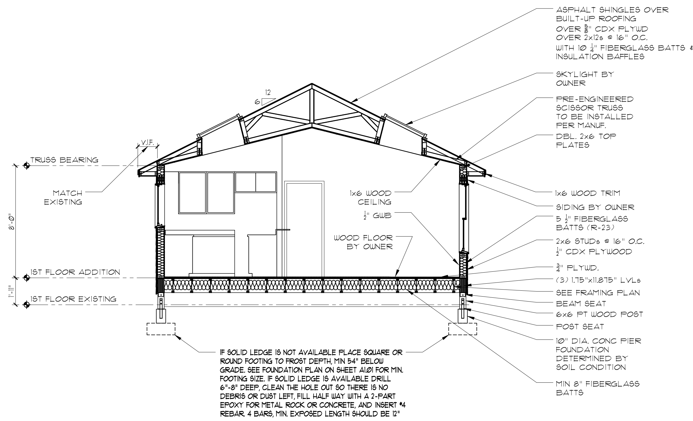
BUILDING SECTION 'A' SCALE: 1/4"=1'-0"
