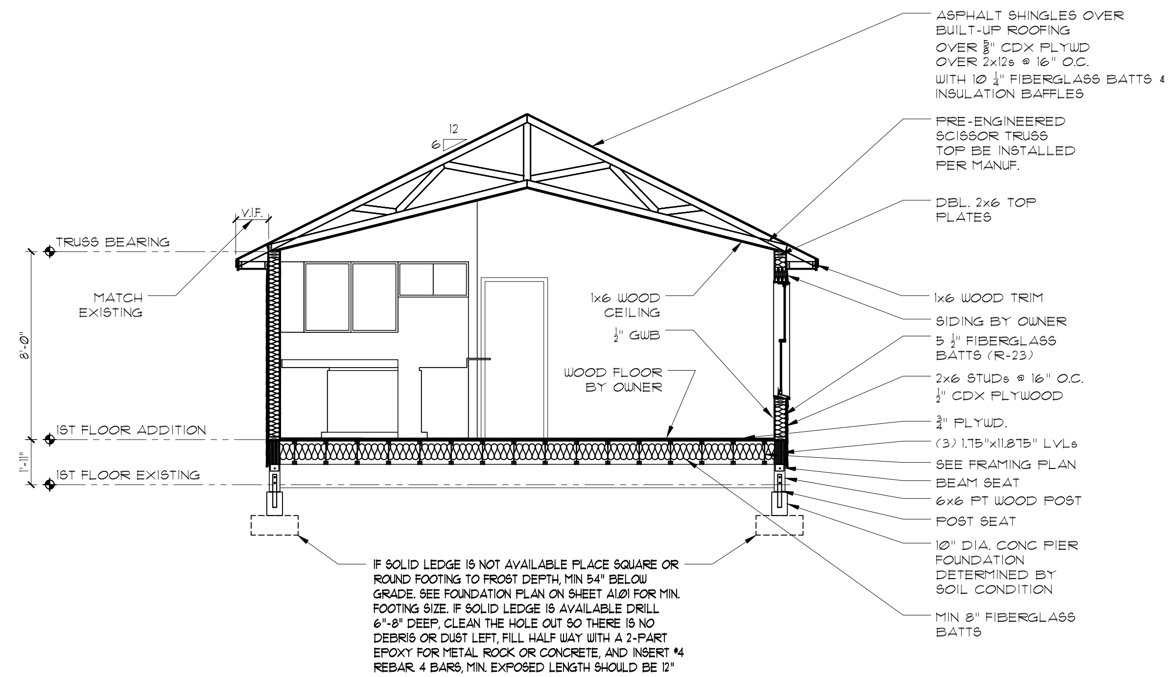
BUILDING SECTION 'B' SCALE: 1/4"=1'-0"
